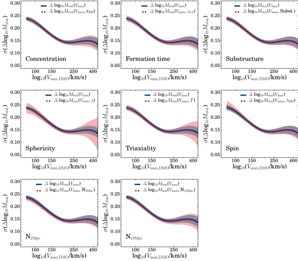
Figure 10.8: As Fig. 10.6 but now with the scatter in stellar mass as a function of V_{\max, \text{DMO}} instead of M_{200, \text{DMO}} . The addition of a dimensionless halo property to V_{\max, \text{DMO}} does not result in statistically more accurate stellar masses.
