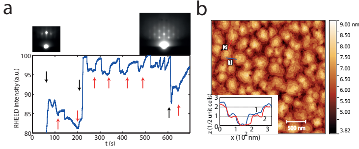
Figure 3.12: (a) RHEED signal vs. time for \text{Nd}_{1.95}\text{Ce}_{0.05}\text{CuO}_4 growth on an annealed (\text{LaAlO}_3)_{0.3}(\text{Sr}_2\text{AlTaO}_6)_{0.7} surface. The black and red arrows represent manual augmentation of the beam intensity, and growth interruption, respectively. The RHEED data in between the arrows show slight oscillatory behavior, typical of the island-like growth exhibited by \text{Nd}_{1.95}\text{Ce}_{0.05}\text{CuO}_4 . The initial substrate surface of annealed (\text{LaAlO}_3)_{0.3}(\text{Sr}_2\text{AlTaO}_6)_{0.7} shows clear two-dimensional spots, while the spotty behavior of the RHEED pattern after growth is another indication of the presence 3D islands. (b) The AFM image of a 30 UC thick \text{Nd}_{1.95}\text{Ce}_{0.05}\text{CuO}_4 film on (\text{LaAlO}_3)_{0.3}(\text{Sr}_2\text{AlTaO}_6)_{0.7} , the surface of which is island-like. The inset shows height steps corresponding with half the c axis lattice parameter of \text{Nd}_{1.95}\text{Ce}_{0.05}\text{CuO}_4 , 6.5 Å.
