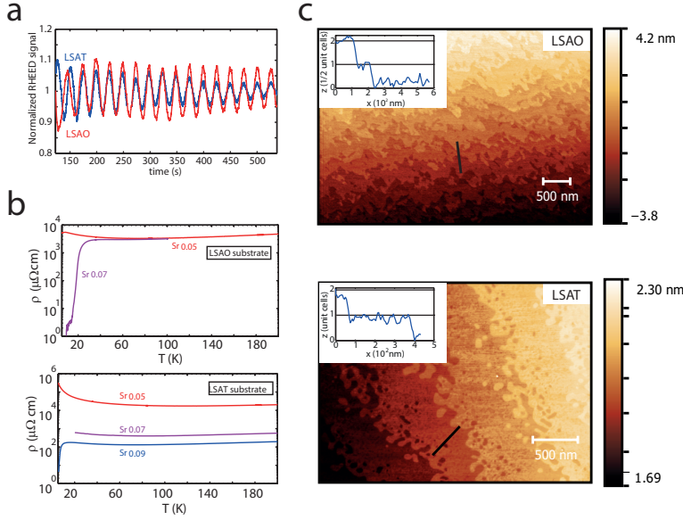
Figure 3.8: (a) Normalized RHEED signal vs. time for \text{La}_{1.95}\text{Sr}_{0.05}\text{CuO}_4 growth on \text{LaSrAlO}_4 (LSAO) and (\text{LaAlO}_3)_{0.3}(\text{Sr}_2\text{AlTaO}_6)_{0.7} (LSAT). The RHEED oscillation amplitude in the former case is preserved over a substantially larger amount of oscillations than in the latter case. (b, top) \rho(T) characteristics for different levels of Sr doping of a 30 UC film grown on \text{LaSrAlO}_4 . For x = 0.05 the film is on the verge of being a superconducting at 4 K. Increasing the doping to x = 0.07 induces a superconducting transition, with a T_{c,\text{mid}} of 20 K. When grown on (\text{LaAlO}_3)_{0.3}(\text{Sr}_2\text{AlTaO}_6)_{0.7} (b, bottom), former two doping levels are insufficient to induce a superconducting transition, for which a doping of x = 0.09 is needed. (c, top) Atomic force microscopy (AFM) scan of an annealed surface of \text{LaSrAlO}_4 , which has double termination. Inset: the steps indicate that the height difference between the next-neighbour terraces is equal to \frac{1}{2} \times c -axis lattice parameter of \text{LaSrAlO}_4 , namely 6.3 Å. Annealed (\text{LaAlO}_3)_{0.3}(\text{Sr}_2\text{AlTaO}_6)_{0.7} (c, bottom) typically shows full UC steps of 3.4 Å.
