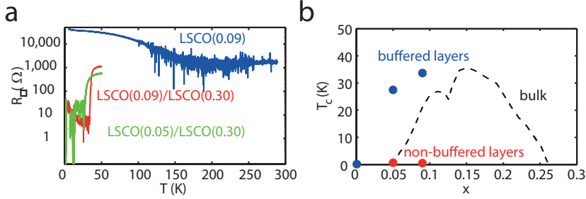
Figure 3.11: (a) R(T) curves of various doping levels of \text{La}_{2-x}\text{Sr}_x\text{CuO}_4 (LSCO) of a total thickness of 7 UC. The unbuffered film shows the expected semiconducting behavior, while the insertion of a buffer layer of 0.30 leads to superconductivity. The doping levels are parenthesized. (b) The T_c values induced in the buffered films are much higher than attainable in the non-buffered films, or bulk material.
