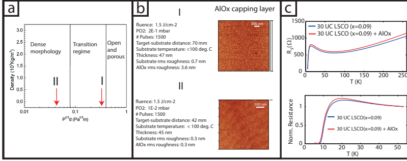
Figure 3.14: (a) Film density vs. \sqrt{pd} for different morphological regimes of \text{AlO}_x , based on Ref.166. For high kinetic energy of the incoming particles, the film is dense, whereas an open and porous film is obtained for low kinetic energies. (b) AFM images of \text{AlO}_x layers I and II grown in the intermediate and dense regime, respectively. Layer I shows a coarsened surface, while layer II shows a flat surface. Both layers I (c,top) and II (c,bottom) do not affect the \text{La}_{2-x}\text{Sr}_x\text{CuO}_4 substantially in T_c .
