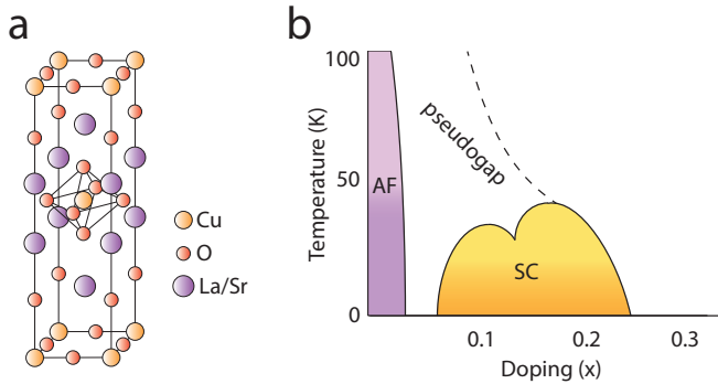
Figure 1.3: (a) The body-centered tetragonal structure of \text{La}_{2-x}\text{Sr}_x\text{CuO}_4 and (b) its phase diagram. Different phases (antiferromagnetic (AF), superconducting (SC) and pseudogap) are present, depending on the temperature and doping.
