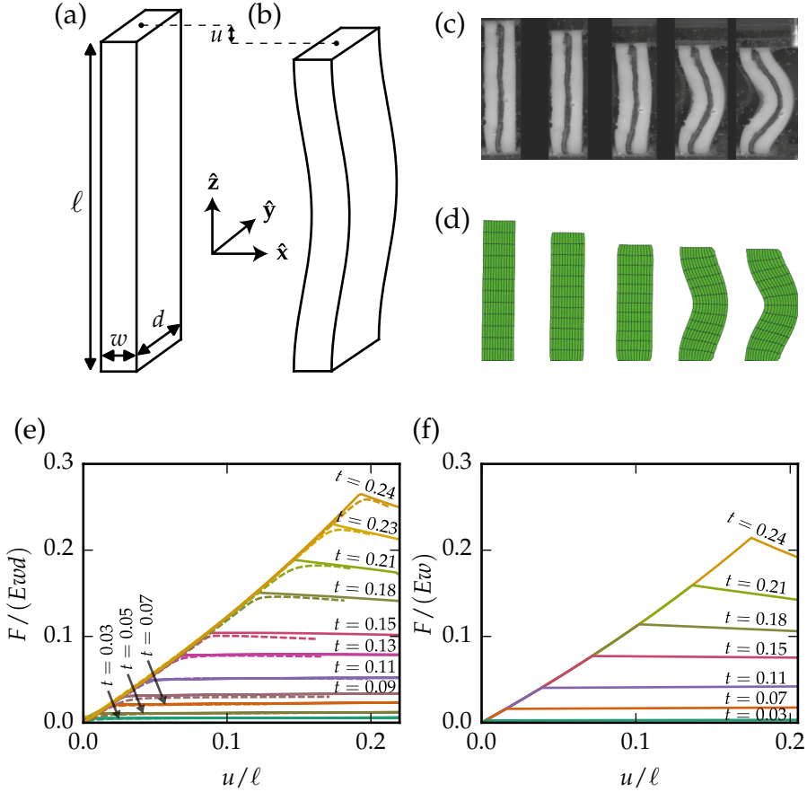
Figure 2.1: Buckling of wide neo-Hookean beams. (a) Sketch of a beam in its initial undeformed state, for which the beam has a rest length \ell , width w and depth d . (b) Applying a compressive displacement u , leads to compression and eventually buckling of the beam. (c-d) Front-view snapshots of (c) the experiment and (d) the simulation for a beam of length \ell = 45 mm, depth d = 35 mm and width w = 11.95 mm, at compressive displacements (from left to right) u = 0 , u = 0.5 u_c , u = 0.99 u_c , u = 1.1 u_c and u = 1.2 u_c . (e-f) Scaled compressive force F/(Ewd) vs. compressive displacement u/\ell for beams of different width for (e) the experiments (dashed lines) and 3D simulations (solid lines) and (f) the simplified 2D simulations. As the effects of gravity are negligible in the experiments and absent in simulations, the choice of the Young's modulus E is irrelevant and we scale the forces by E .
