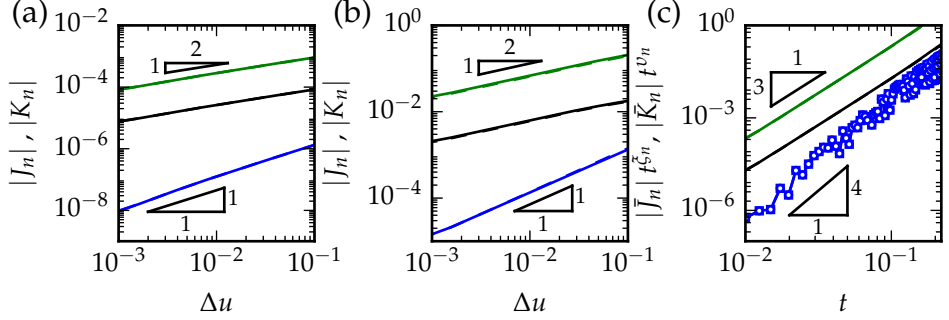
Figure 2.7: Dependence of the spatial nominal shear strain and stress profiles on \Delta u and t , obtained by FEM simulations. In black, blue and green we have plotted the post-buckling profile coefficients J_n (solid lines) and K_n (dashed lines), corresponding to order n = 0 , n = 1 and n = 2 respectively. (a-b) We have plotted |J_n| and |K_n| as function of \Delta u for (a) a slender beam ( t = 0.02 ) and (b) a thick beam ( t = 0.15 ). (c) Dependence of J_n and K_n on the beam's aspect ratio t .
