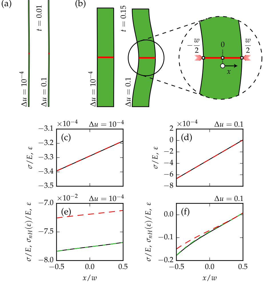
Figure 2.5: Beam shapes, stress-strain relation and stress and strain profiles. (a-b) Beam shapes for (a) a slender ( t = 0.01 ) and (b) wide ( t = 0.15 ) beam at excess strains of \Delta u = 1 \times 10^{-4} and \Delta u = 0.1 . We track the nominal stress and strain profiles as a function of the transverse coordinate x at the central cross section of the beam, depicted by the horizontal red lines. (c-d) Rescaled uniaxial nominal stress (solid black) and strain (dashed red) profiles for a slender beam ( t = 0.01 ) at an excess strain of (c) \Delta u = 1 \times 10^{-4} and (d) \Delta u = 0.1 . (e-f) Rescaled uniaxial nominal stress and strain profiles for a wide beam ( t = 0.15 ) at an excess strain of (e) \Delta u = 1 \times 10^{-4} and (f) \Delta u = 0.1 . The green dash-dotted lines correspond to \sigma_{\text{NH}}(\epsilon)/E , obtained by applying the neo-Hookean stress-strain relation in Eq. (2.10a) to the strain profile obtained from FEM simulations.
