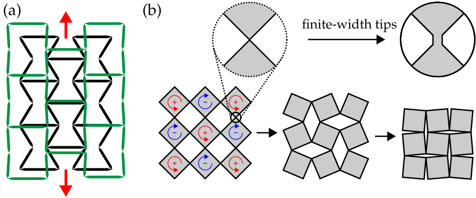
Figure 1.2: Auxetic metamaterials. (a) Structure with inverted honeycomb cells, which expands (shrinks) in the lateral direction when stretched (compressed) [21]. (b) A collection of squares linked at their tips exhibits a free hinging motion (indicated by the coloured arrows), which allows the structure to uniformly contract or expand [20]. Zoomed areas: The sharp tips localize bending and approximate ideal hinges (left). Finite-width tips can be regarded as beams (right).
