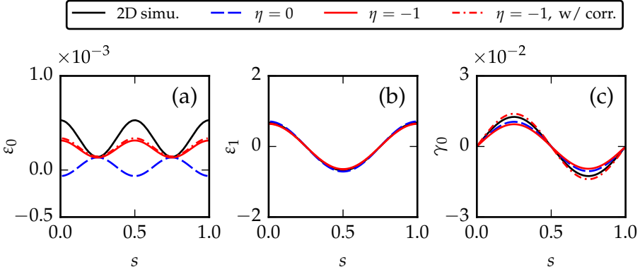
Figure 2.9: Mindlin-Reissner strains as a function of s , for four different models. We consider a wide ( t = 0.1 ) beam which is compressed to an axial displacement of u/u_c = 1.06 . We show results for 2D simulations (solid black), and compare them to numerical solutions to our beam model in Eqs. (2.38) for \eta = 0 (dashed blue) and \eta = -1 (solid red). Finally, we also show numerical solutions to an extension of our beam model in Eqs. (2.48) discussed in section 2.6.3 (dash-dotted red). (a-c) We have respectively plotted the compressive, bending and shear Mindlin-Reissner strain along the beam.
