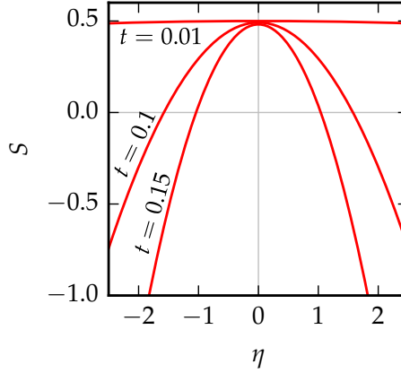
Figure 2.10: Post-buckling slope as a function of the nonlinearity \eta . Using Eq. (2.44) we have plotted S(\eta) for t = 0.01 , t = 0.1 and t = 0.15 . The curves show that the post-buckling slope is quadratic in \eta and that the post-buckling slope does not exceed S = 1/2 .
