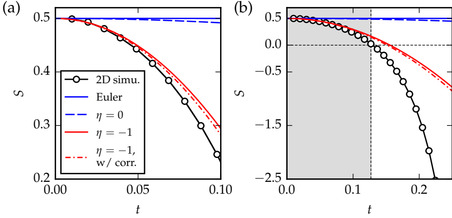
Figure 2.8: Post-buckling slope S as function of the beam width-to-length ratio t , for five different models. In the Euler limit S = 1/2 , while in 2D simulations (open circles) S varies with t . Solutions to our model, given by Eq. (2.44), are shown for \eta = 0 (dashed blue) and \eta = -1 (solid red). Finally, we also show data for an extension of our model discussed in section 2.6.3 (dash-dotted red). (a-b) Panel (a) shows a close-up for 0 < t < 0.10 and panel (b) shows a wider range of width-to-length ratio ( 0 < t < 0.25 ). The shaded region indicates the cross-over to subcritical buckling ( S < 0 ) for the 2D simulations.
