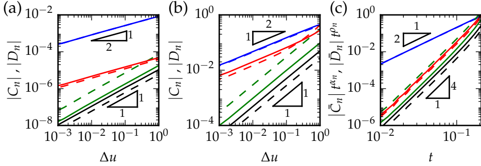
Figure 2.6: Expansion of the nominal strain and stress profiles obtained by FEM simulations, according to Eqs. (2.11-2.12). We plot the post-buckling profile coefficients C_n and D_n in each order as a function of \Delta u and t . In black, blue, green and red we have plotted C_n (solid lines) and D_n (dashed lines), corresponding to the order n = 0, n = 1, n = 2 and n = 3 respectively. (a-b) We have plotted |C_n| and |D_n| as function of \Delta u for a (a) slender beam ( t = 0.02 ) and (b) thick beam ( t = 0.15 ). (c) Dependence of C_n and D_n on the beam's aspect ratio t .
