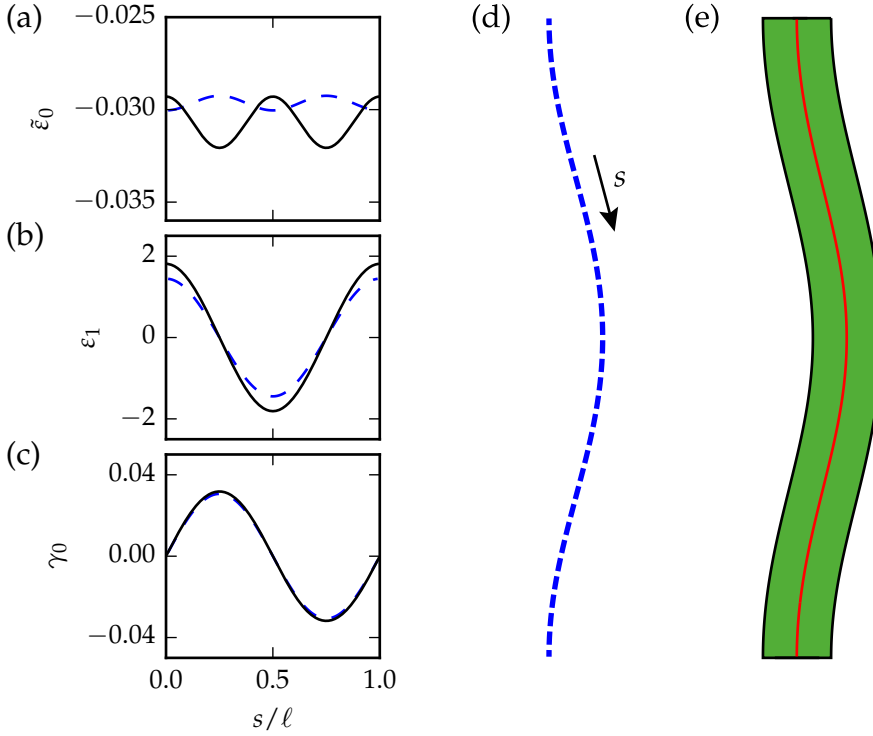
Figure 2.4: Mindlin-Reissner strains and corresponding beam shapes for a beam ( t = 0.1 ) which is uniaxially compressed to a displacement of u/u_c = 1.3 . (a–c) The solid black curves depict data for the Mindlin-Reissner strains obtained from FEM simulations, and the blue dashed curves are numerical solutions of the linear elastic wide beam model [Eqs. (2.9)]. As a function of the curvilinear coordinate s , we show (a) the compressive strain, (b) the bending strain, and (c) the shear strain. (d) Shape of the central axis as predicted by the linear beam model. We have obtained this shape by the integration of the horizontal and vertical component of the displacement gradient with respect to s , respectively given by \lambda \cos(\theta + \chi) and \lambda \sin(\theta + \chi) [41]. (e) Beam shape and associated central axis (solid red) obtained from 2D FEM simulations.
