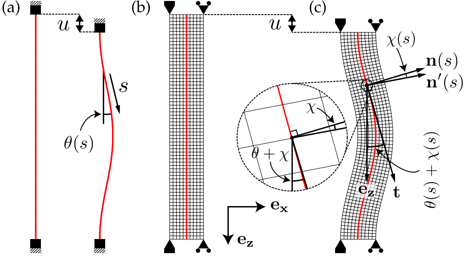
Figure 2.3: Kinematic description of a slender ( t = 0^+ ) and wide beam (here, t = 0.15 ). Both beams are compressed equally by a displacement u . (a) The shape of an undeformed (left) and buckled (right) slender beam. We obtain the buckled state by solving Euler’s elastica [Eq. (2.6)] for clamped boundary conditions at both ends. The kinematic description of a slender beam is governed by the rotation angle \theta(s) . (b) Snapshot from a 2D simulation of a wide neo-Hookean beam in its undeformed state, where each square represents a simulation element. We impose clamped boundary conditions at both ends of the beam, but allow free lateral expansion along the x -direction at top and bottom boundaries. The superimposed, red, solid line depicts the central axis of the beam as obtained from FEM simulations accordingly. (c) Snapshot from the same simulation as in (b), depicting the beam in its deformed state. The deflection of the central axis under a compressive displacement u is described by a combination of the rotation angle, \theta(s) , and shear angle, \chi(s) along the curvilinear coordinate of the beam as indicated. For a precise definition of \theta(s) and \chi(s) as well as the vectors \mathbf{n}(s) , \mathbf{n}'(s) and \mathbf{t}(s) , see the main text.
