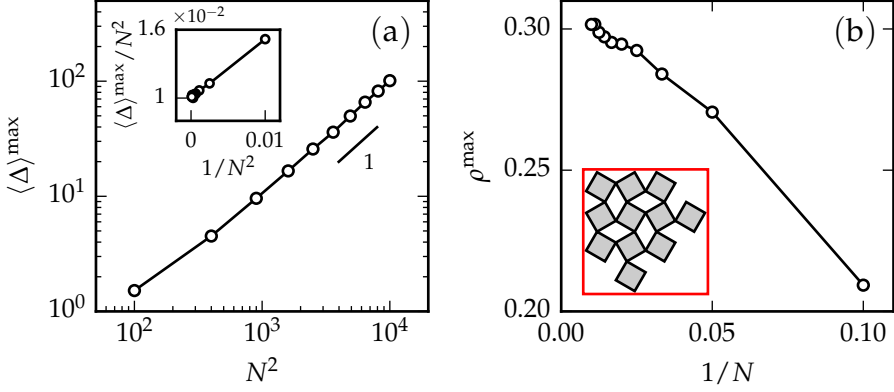
Figure 3.13: Peak behaviour of \langle \Delta \rangle(\rho) . For the data shown in Fig. 3.12, we have determined the value and location of the peak with system size. (a) The value of peak grows linearly with N^2 for large N (log scale, slope 1), implying that \langle \Delta \rangle_{\max} \sim N^2 . Inset (linear scale): For small N , the scaling \langle \Delta \rangle_{\max} \sim N^2 exhibits finite size corrections proportional to 1/N^2 . (b) The peak location tends to a constant as 1/N . Inset: Unit cell to understand the value of \rho_{\infty} (see main text).
