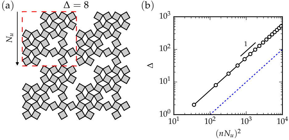
Figure 3.18: Excess modes in nN_u \times nN_u systems built by the periodic tiling of a N_u \times N_u unit cell ( n = 1, 2, 3, \dots ). (a) System corresponding to n = 2 , resulting in \Delta = 8 . The quads enclosed within the dashed red region display the unit cell. (b) The number of excess zero modes grows proportionally with (nN_u)^2 (open circles, solid line). We display data up to n = 16 ( nN_u = 96 ). The blue dashed line represents the asymptotic growth of excess zero modes in randomly diluted systems as function of system size.
