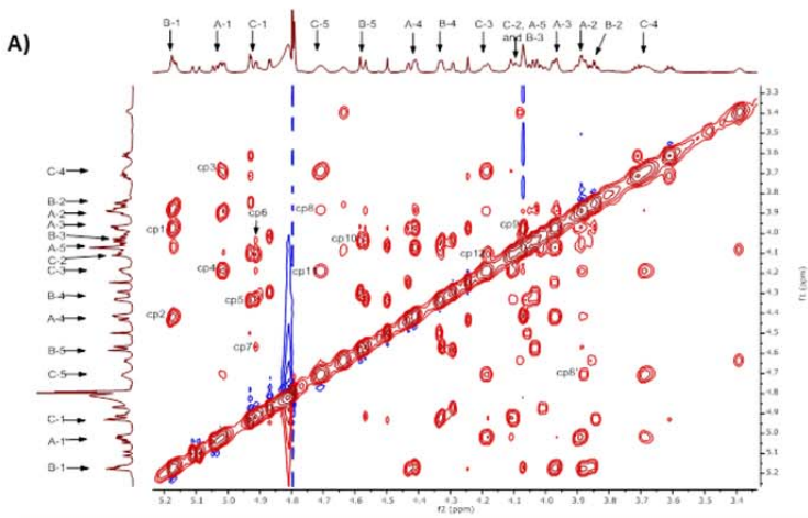
Figure 7.3 NOE spectrum of dodecamer 4 (with selected NOESY interactions) and native SP1 [17b]
