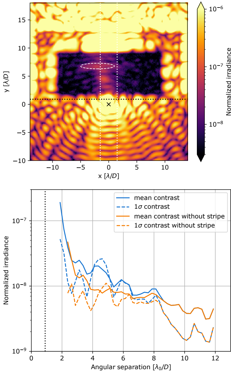
Figure 8.9: The coronagraphic normalized irradiance image and the normalized radial irradiance. The known incoherent ghost, outlined with the dotted white ellipse, has been excluded from the image before taking the radial profile. This curve has been corrected for the coronagraphic throughput of an off-axis source.
