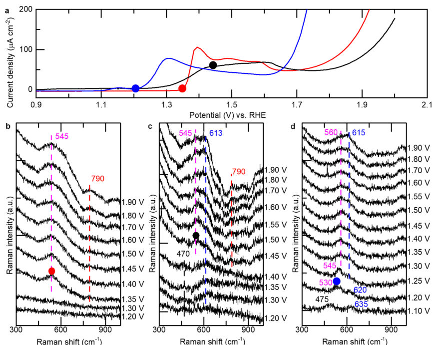
Figure 4. In situ SERS of gold oxidation. (a) LSV for electrocatalytic water oxidation from 0.9 to 2 V vs RHE at 50 mV/s on the gold electrode in Ar-saturated 0.1 M \text{H}_2\text{SO}_4 (red line), \text{Na}_2\text{SO}_4 (black line), and \text{NaOH} (blue line) solution. (b–d) SERS of gold oxidation in 0.1 M \text{H}_2\text{SO}_4 (b), \text{Na}_2\text{SO}_4 (c), and \text{NaOH} (d). Oxidation potentials were recorded on the RHE scale. Solid circles represent the points where the \nu(\text{Au}-\text{O}) vibration becomes visible in 0.1 M \text{H}_2\text{SO}_4 (red circle), \text{Na}_2\text{SO}_4 (black circle), and \text{NaOH} (blue circle) solutions.
