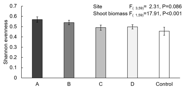
Figure S 3.5 Mean Shannon evenness (±SE) of Jacobaea vulgaris leaf metabolomes of plants grown with inocula from 4 different sites (A, B, C, D) and in 100% sterilized soil with shoot biomass as covariate. The results of an analysis of variance (ANOVA) testing for the effects of site, plots nested within site, and shoot biomass is also presented. For this analysis the 100% sterilised soil treatment was removed
