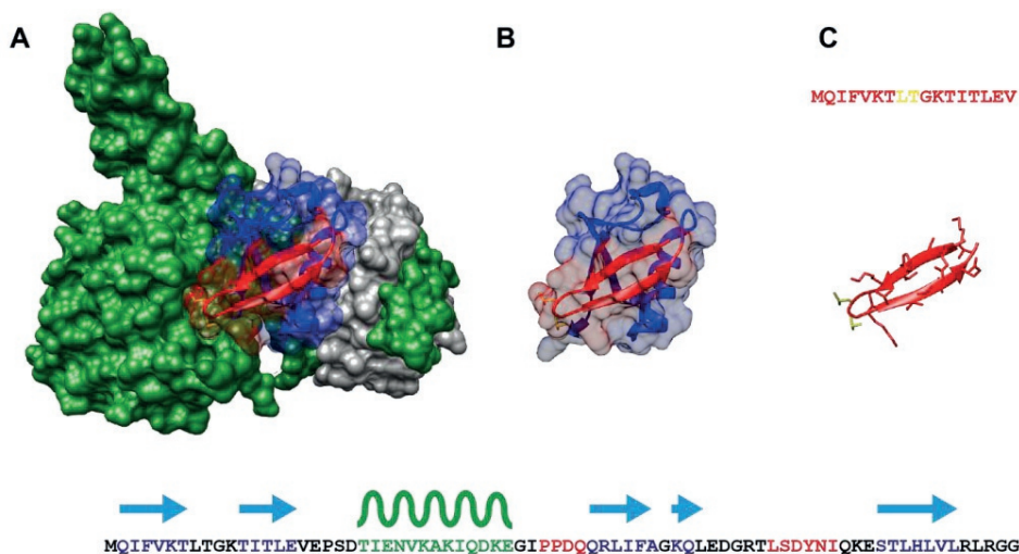
Figure 1: Structure of Ub binding to UCHL5/Rpn13. A: X-ray structure of UCHL5 (in green) bound to Ub-PRG (in blue) and Rpn13 (grey) (PDB: 4UEL). Location of the binding pocket for Lue8 and Thr9 of Ub is represented in orange and the first \beta -sheet of Ub is shown in red. B: Isolated structure of Ub showing the orientation of the first \beta -sheet (in red). The sequence of Ub showing different secondary structures is shown below. C: Structure of the \beta -sheet peptide of Ub encompassing residues 1 to 17 in which the important residues, namely Leu8 and Thr9, are highlighted in yellow. D: Sequence of full-length Ub showing residues that comprises the \beta -sheet (blue arrows) and the \alpha -helix (green curves). Residues that constitute the connecting loops are highlighted in red.
