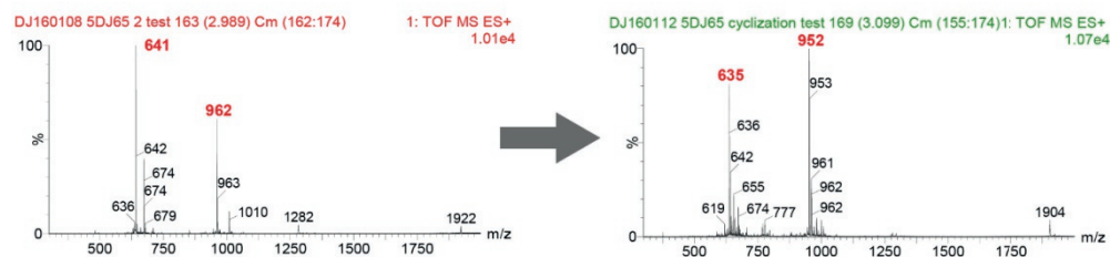
Figure S1: Cyclization of Ub (1-17) peptide. A: Schematic illustration of cyclization procedure where the N- and the C-terminus of the peptide is conjugated together using peptide coupling procedure. B: UV chromatogram from the LC/MS measurement of the peptide before (left) and after (right) cyclization procedure. C: Mass spectrometric signals of Ub (1-17) peptide before (left) and after (right) the completion of cyclization.
