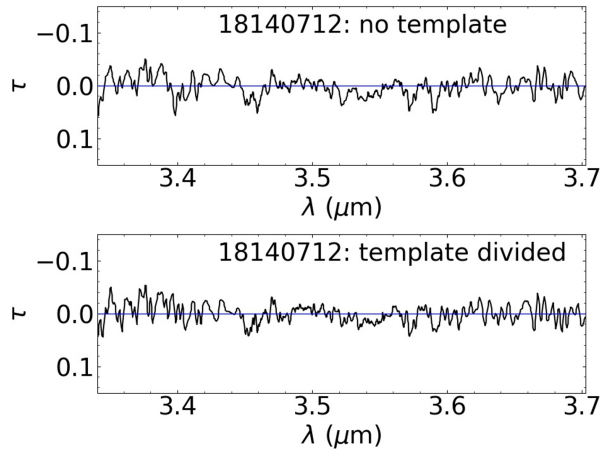
Figure 5.2: Optical depth spectra taken towards the field star, 18140712 (Boogert et al. 2011). No observable 3.537\text{ }\mu\text{m} \text{CH}_3\text{OH} feature is present in either panel, whereas the feature was present in Boogert et al. (2011). The choice of baseline may be the cause of such discrepancy. The blue line indicates \tau=0 .
