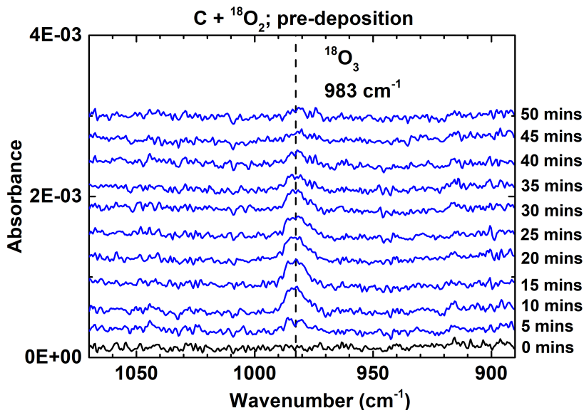
Figure 2.12: RAIR spectra acquired after pre-deposition of atomic C and {}^{18}\text{O}_2 on a 10 K surface (exp. 2). 10 L of {}^{18}\text{O}_2 is first deposited, followed by carbonation for 50 minutes. The increase and subsequent decrease of the {}^{18}\text{O}_3 band is highlighted. RAIR spectra are offset for clarity.
