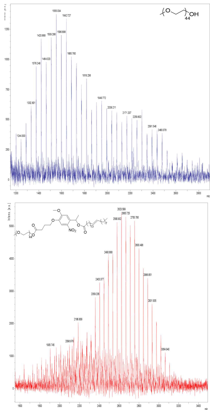
Figure S2. Maldi-TOF spectrum of mPEG 2000 and 1 . (The mass difference between mPEG 2000 and 1 is 630 g/mol which is the exact mass value of the extra part of nitrobenzyl-nervonic acid).
