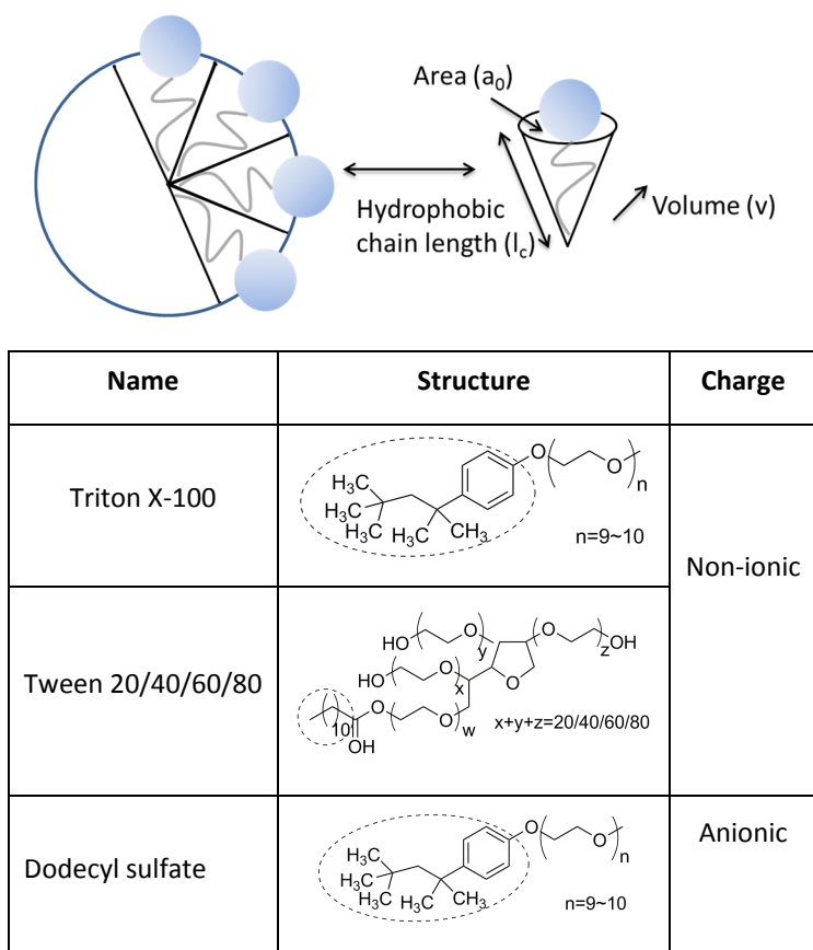
Figure 12. The required geometry of molecules for micelle formation (top) and the structure of some common micelle-forming detergents (bottom); the dash line circled part is hydrophobic component.
