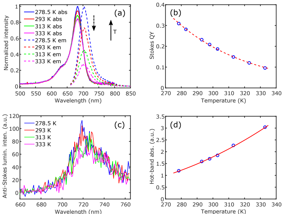
Figure 4.3: Optical characterization of Seta 670. (a) Absorption and Stokes fluorescence emission spectra of 1 \mu M Seta 670 in methanol at different temperatures. The absorption spectra have been normalized relative to the highest absorption spectrum and the emission spectra have been normalized relative to the highest emission spectrum. The excitation wavelength for the emission spectra was 650 nm. (b) Quantum yield of Stokes fluorescence of Seta 670 as a function of temperature. The dashed red line is an empirical exponential fit to the experimental data. (c) Anti-Stokes luminescence spectra of Seta 670 at different temperatures ( \lambda_{\text{exc}} = 775 nm). (d) Hot-band absorption efficiency as a function of temperature ( \lambda_{\text{exc}} = 775 nm). The red line shows an exponential fit to equation 4.1.
