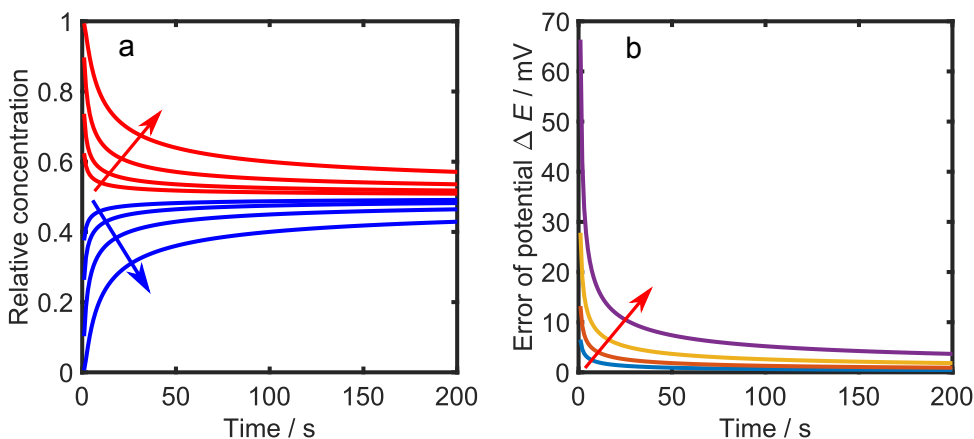
Figure S3.1: Control of the redox potential relies on the diffusion of the electron mediator. a) Calculated concentration evolution at positions with different distances to the electrode (10 μm, 20 μm, 40 μm and 80 μm) after the mid-point potential is applied at t = 0 to a solution of \text{PES}_{\text{ox}} . The arrows indicate increasing distance. The concentrations of oxidized (red) and reduced (blue) PES are scaled by the original concentration of \text{PES}_{\text{ox}} . b) Calculated error of redox potential compared to the applied potential at different distances away from the electrode (10 μm, 20 μm, 40 μm and 80 μm) after the mid-point potential is applied at t = 0 . The arrow indicates increasing distance. The diffusion coefficient of PES in the aqueous buffer is assumed to be 5 \times 10^{-6} \text{ cm}^2/\text{s} in the calculations.
