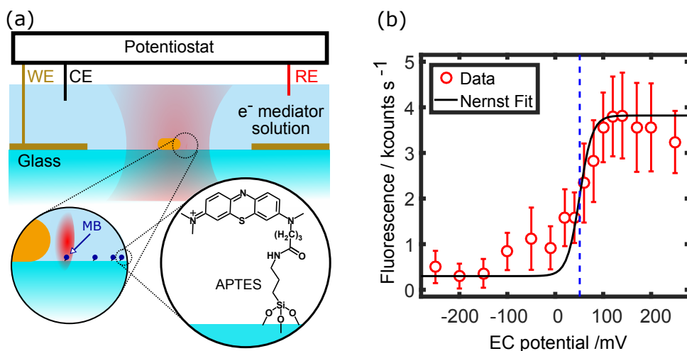
Figure 3.2: Electrochemistry with fluorescent readout. (a) Scheme of the combined electrochemical-confocal setup and sample (WE: working electrode, CE: counter electrode, RE: reference electrode). Individual AuNRs (not to scale) and MB molecules were immobilized on the glass surface. Phenazine ethosulfate mediates electron transfer between MB molecules and the gold film controlled via the potentiostat. (b) Ensemble fluorescence response of \sim 260 unenhanced MB molecules to the electrochemical potential, showing the controlled switching from the reduced state at low potentials to the oxidized state at high potentials. The black curve is a fit using the Nernst equation and the dashed line illustrates the obtained mid-point potential ( 51 \pm 4 mV).
