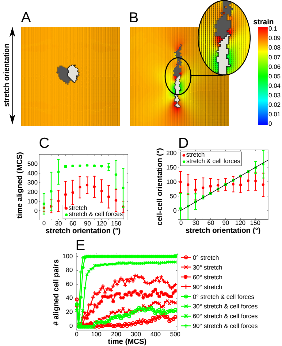
Figure 3.2: Response of two adjacent cells to static stress. (A) Non-contractile cell pair on substrate stretched along 0° at 500 MCS; (B) contractile cell pair on substrate stretched along 0° at 500 MCS; (A-B) colors: principal strain magnitude; orientation and length of black line pieces: orientation and magnitude of principal strain; (C) fraction of time a cell pair is aligned, averaged over n = 100 simulations, upper bars for contractile cells and lower bars for non-contractile cells; (D) angle of the line connecting the center of masses as a function of stretch orientation at 500 MCS, averaged over n = 100 simulations, contractile cells follow the extra plotted linear line piece. (C-D): error bars: standard deviations; (E) time series of the number of cell pairs that are aligned on stretched substrates with different stretch orientations; symbols are circle: 0°, cross: 30°, star: 60°, plus: 90°, upper lines for contractile cells and lower lines for non-contractile cells. Color coding (C-E): red: non-contractile cells; green: contractile cells.
