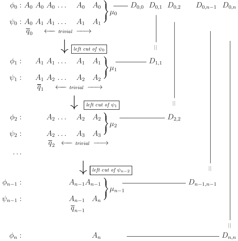
Figure 9: An illustration of our reasoning that res(\phi) = res(\psi) . Here \phi_n = lcut(\psi_{n-1}) .
