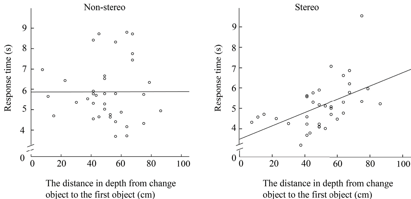
Fig 10. Response time as a function of the absolute depth from the changed object to the first object (the object closest to the camera). (a) Non-stereo viewing condition, (b) stereo viewing condition.
