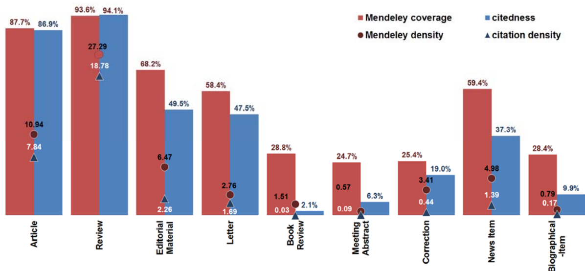
Figure1. Mendeley coverage and density, citedness and citation density per document type. Document types appear in order of frequency: article (N=1,132,428), review (N=64,734), editorial material (N=60,533), letter (N=29,410), book review (N=21,710), meeting abstract (N=13,071), correction (N=9,817), news item (N=4,880) and biographical item (N=2,302). Document types that occurred less than 2,300 times were not analyzed.
