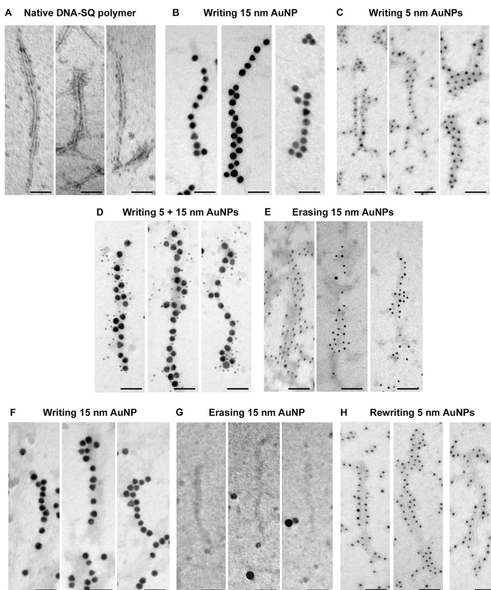
Figure 1. Conventional TEM images of SQ/SQ-DX multicomponent supramolecular polymers with and without AuNPs stained with uranyl acetate (0.8%): A) SQ supramolecular polymers (50 \mu\text{m} ) bearing SQ-D1 (0.5 \mu\text{m} ) or SQ-D2 (0.5 \mu\text{m} ), B) SQ supramolecular polymer written on with 15 nm AuNPs (Au15-D3, 25 nm), C) and 5 nm AuNPs (Au5-D4, 250 nm). D) Dual writing of both 5 and 15 nm AuNPs (Au15-D3, 70 nm and Au5-D4, 540 nm) on independent DNA strands (SQ-D1 and SQ-D2, both 0.25 \mu\text{m} ), E) and selective erasing of 15 nm AuNPs using DD5. F) SQ supramolecular polymers written on with 15 nm AuNPs (Au15-D3, 25 nm), G) which are erased by using an equimolar amount of DNA displacement strand (DD5), H) and are rewritten on with 5 nm AuNPs (Au5-D3, 125 nm). Scale bars 50 nm.
