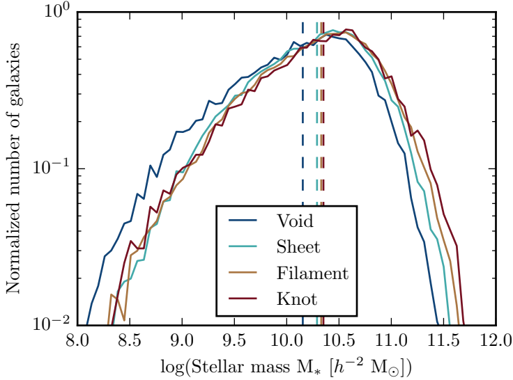
Figure 3.2: The normalized number of galaxies in each cosmic environment as a function of stellar mass M_* . Each vertical dashed line shows the mean of the M_* distribution. The distributions show that galaxies in denser cosmic environments tend to have slightly higher stellar masses.
