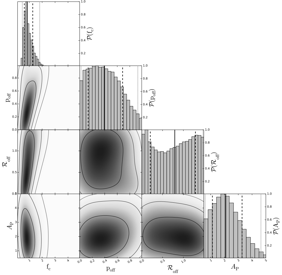
Figure 2.9: Posterior distribution of the normalisation of the mass-concentration relation f_c , of the mis-centring parameters p_{\text{off}} and R_{\text{off}} and of the amplitude of the point mass A_P . The contours indicate the 1, 2, 3 sigma confidence regions. The dashed vertical lines and the dotted vertical lines correspond respectively to the 1 and 2 sigma marginalised confidence limits. These are the constraints from a joint halo model fit of the ESD signal in the 6 luminosity bins using BCG as the group centre. The range in each panels reflect the priors used for the different parameters.
