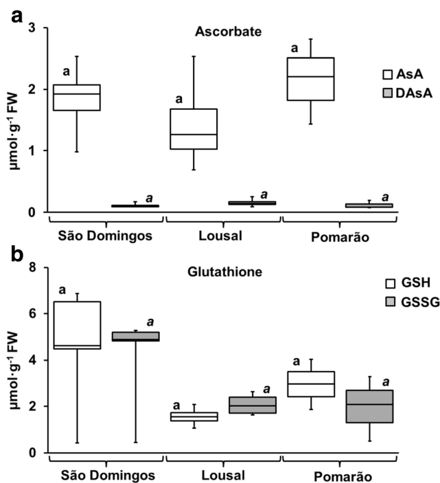
Fig. 3 a Concentrations of reduced (AsA) and oxidised (DAsA) ascorbate and b reduced (GSH) and oxidised (GSSG) glutathione in shoots of C. monspeliensis from the different studied areas. Box plot data distribution (min, Q1, median, Q3, max) for each parameter is indicated for each studied area. Black bars show the maximum and minimum values in each studied populations. Values with same letter (lowercase letter, or lowercase italic) indicate that there are no significant differences for each parameter among studied areas ( p < 0.05)
