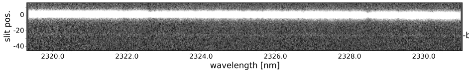
Figure 4.1: An example of a two-dimensional spectrum from detector 3, after the basic data reduction steps and cropped to the relevant slit positions. The bright band is the spectral trail of the star. Twenty-six pixels below, the faint trail of the companion can be seen (marked with b ).
