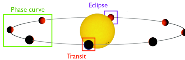
Figure 1.3: Transiting exoplanets provide three distinct methods for characterising the atmosphere of the planet. Image credit: Ernst de Mooij
