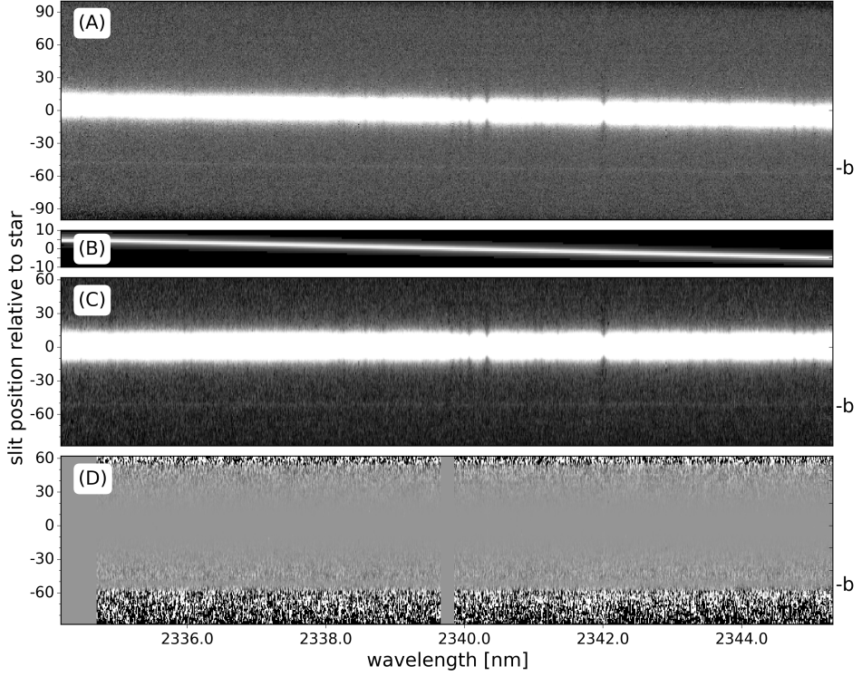
Figure 5.2: Illustration of the data analysis steps from detector 4 as observed on 2014-05-29. The y-axes depicts the slit position relative to the average centroid of the stellar profile. The companion position is indicated by a 'b' on the right-hand axes. The greyscales were adjusted individually for each array with an IRAF-like z-scale algorithm. Top to bottom: (A) The average two-dimensional spectrum, where the individual AB-combined frames were weighted by the FWHM of the stellar profile as given in Fig. 5.1. (B) A map of the stellar profiles made by fitting the continuum of each of the central rows. (C) The spatial spectra, extracted by applying the stellar profile map as weights for each slit position. Each row corresponds to an optimally extracted spectrum for the given slit position. (D) The residual spatial spectra after removing the scaled stellar spectrum, dominated by telluric lines.
