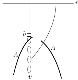
Fig. 6. Schematic representation of the event F'_n(v; A) \cap \{b \in \mathcal{P}_A\} .
