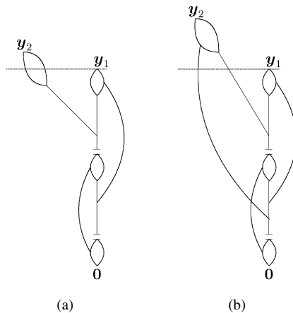
Fig. 8. Examples of diagrams that contribute to R^{(2)}(y_1, y_2) and Q^{(2)}(y_1, y_2) .
