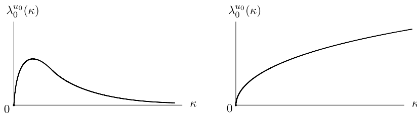
Fig. 3. Qualitative picture of \kappa \mapsto \lambda_0^{u_0}(\kappa) in the weakly, respectively, strongly catalytic regime.
