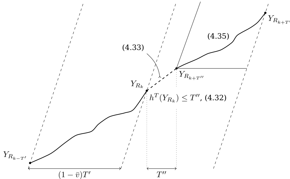
Figure 4: Illustration of a good record time R_k . Note the validity of the conditions (4.32), (4.33) and (4.35).
