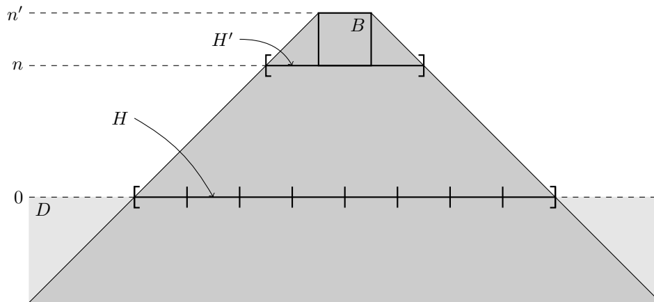
Figure 6: Box B and lower halfplane D as in Theorem C.1. The dark gray area corresponds to the cone associated with B , containing the separating segments H and H' .
