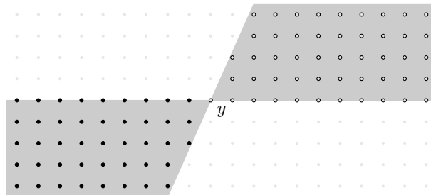
Figure 3: An illustration of the sets \mathcal{Z}(y) (represented by white circles) and \bar{\mathcal{Z}}(y) (represented by filled black circles), with y = (x, n) \in \mathbb{Z}^2 .
