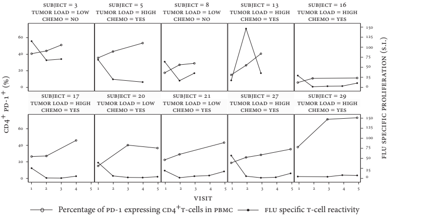
Figure s7 Individual plots, showing T-cell responsiveness against FLU within LST. At baseline, positive responsiveness (s.i. \geq 3 ) is seen in all patients. A severe drop in T-cell responsiveness occurs upon EBRT (except for subject 13) and slight rebound 6-9 weeks after completion of EBRT in 6 cases. Except for ID13, the strong decrease in T-cell responsiveness occurred concurrently with an increase in PD-1 expression on CD4 + T-cells. Visit 1: baseline. Visit 2: after 15 fractions of EBRT. Visit 3: 3 weeks after EBRT. Visit 4: 6 weeks after EBRT. Visit 5: 9 weeks after EBRT
