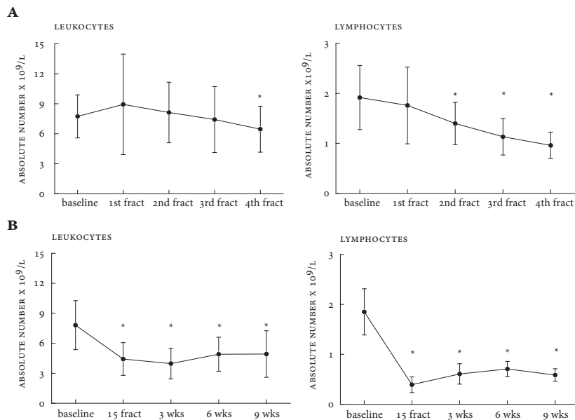
Figure 2 (Chemo)radiotherapy induced reduction in the absolute numbers of leukocytes and lymphocytes. (A) Time course of changes in the absolute number of leukocytes and lymphocytes before (baseline) treatment, and during the first 5 days of fractionized radiotherapy. (B) Time course of changes in absolute number of leukocytes and lymphocytes before (baseline), during (15 fractions) and after (chemo)radiotherapy (3, 6 and 9 weeks after completion). Data are expressed as mean \pm SD. * p < 0.05 .
