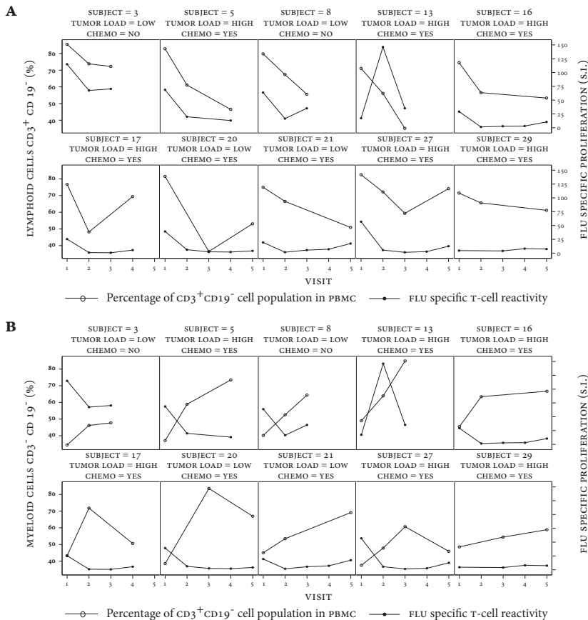
Figure S5 T-cell responsiveness against FLU within LST, presented for 10 individual patients showing high responsiveness at baseline, severe drop upon (chemo)radiotherapy (except for subject 13) and slight rebound 6-9 weeks after completion of EBRT in 6 cases. The strong decrease in T-cell responsiveness occurred concurrently with a decrease in percentage of circulating CD3^+CD19^- lymphoid cells ( A ), and an increase in percentage of circulating CD3^+CD19^- myeloid cells ( B ) in 9 of the 10 patients. Visit 1: baseline. Visit 2: after 15 fractions of EBRT. Visit 3: 3 weeks after EBRT. Visit 4: 6 weeks after EBRT. Visit 5: 9 weeks after EBRT.
