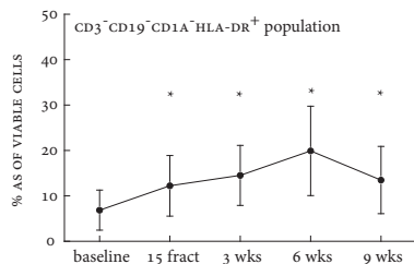
Figure s4 The effect of (chemo)radiotherapy on the percentage of circulating CD3^{-}CD19^{-}CD1A^{-}HLA-DR^{+} population (A) and on the subpopulation of monocytes expressing both CD14 and CD11b (B). Data is expressed as percentage of viable cells. * p < 0.05 with respect to baseline.
