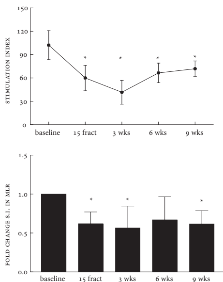
Figure 4 (Chemo)radiotherapy impairs the ability of antigen presenting cells to stimulate allogeneic T-cells. Antigen presenting capacity of PBMCs as determined in a mixed lymphocyte reaction (MLR) in the blood samples from 10 patients are plotted over time. Treatment-induced changes in lymphocyte reactions as observed in the MLR based on (A) Stimulation Index (S.I., expressed as mean \pm SEM) and (B) expressed as the fold changes (mean \pm SEM) of these S.I. over baseline. Time point include baseline, after 15 fractions of EBRT, and at 3, 6 and 9 weeks after completion of EBRT. * p < 0.05 with respect to baseline.
