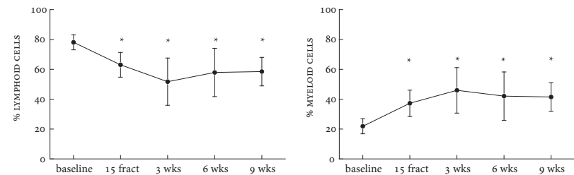
Figure 5 (Chemo)radiotherapy alters the relative frequencies of circulating myeloid and lymphoid cells. (A) Percentages of lymphoid cells ( CD3^{+}CD19^{-} ) and myeloid cells ( CD3^{-}CD19^{-} ) of viable cells as measured by flow cytometry. Mean percentages are shown for 10 patients with a complete follow-up at different time points, including baseline, after 15 fractions of EBRT, and at 3, 6 or 9 weeks after completion of EBRT. Percentages are expressed as mean \pm SD. (B) Fold changes in lymphoid and myeloid cells over baseline. Fold changes are expressed as mean \pm SEM. * p < 0.05 with respect to baseline.
