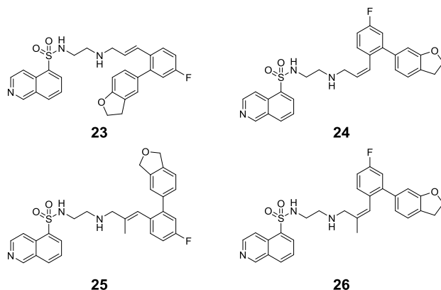
Figure 4. Suggested isoquinolinesulfonamide inhibitors selective for FLT3.
