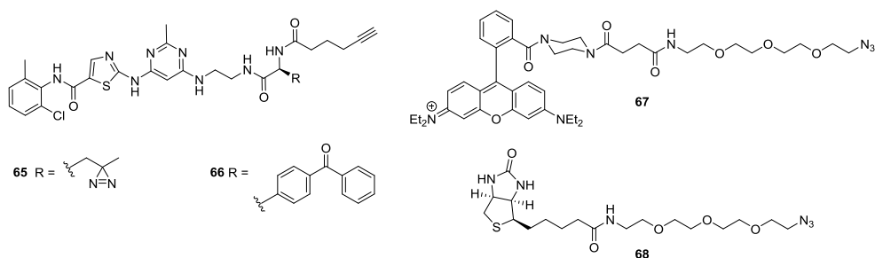
Figure 18. Structures of two-step bioorthogonal photoreactive-group containing dasatinib-probes 65 and 66 . Rhodamine-N 3 ( 67 ) and biotin-N 3 served as the ligation reagents for visualization and pull-down of targets, respectively.
