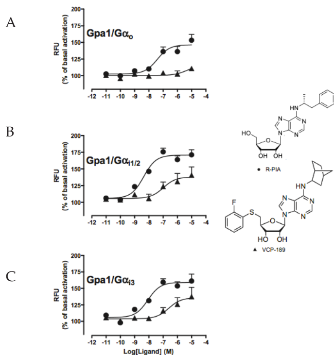
Fig. 1. Influence of G protein subtype on R-PIA and VCP-189 response. Yeast strains expressing the adenosine A_1 receptor with G_{\alpha 1}/G_{\alpha o} (A), G_{\alpha 1}/G_{\alpha i1/2} (B), or G_{\alpha 1}/G_{\alpha i3} (C) were incubated with a range of ligand concentrations for 18 to 24h. Ligand response is expressed in relative fluorescence unit (RFU) corrected for the fluorescence in the absence of ligand. Data points represent mean \pm SEM obtained from three to five experiments performed in duplicate. Reproduced with permission from [15].
