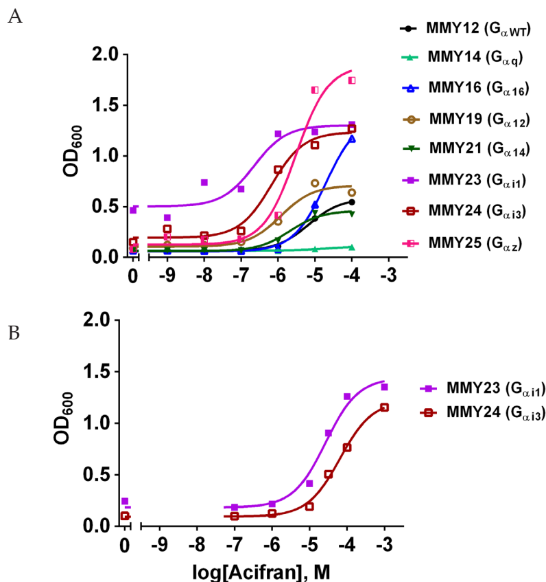
Fig. 2. Concentration-effect curves from liquid assay experiments. (A) Curves are shown of the wild-type receptor hHCA 2 in the different yeast strains: MMY25 ( G_{\alpha z} ), MMY23 ( G_{\alpha i1} ), MMY24 ( G_{\alpha i3} ), MMY16 ( G_{\alpha 16} ), MMY19 ( G_{\alpha 12} ), MMY12 ( G_{\alpha WT} ), MMY21 ( G_{\alpha 14} ), MMY14 ( G_{\alpha q} ) responding to the hHCA 2 agonist nicotinic acid. (B) The wild-type receptor hHCA 3 in the different strains: MMY23 ( G_{\alpha i1} ) and MMY24 ( G_{\alpha i3} ) responding to the hHCA 2 /hHCA 3 agonist acifran. The hHCA 3 receptor was not activated in other strains, and, hence, no further curves are shown. The assays were performed in YNB-NA-ULH medium. A representative experiment is shown (of a total of n = 3 ).
