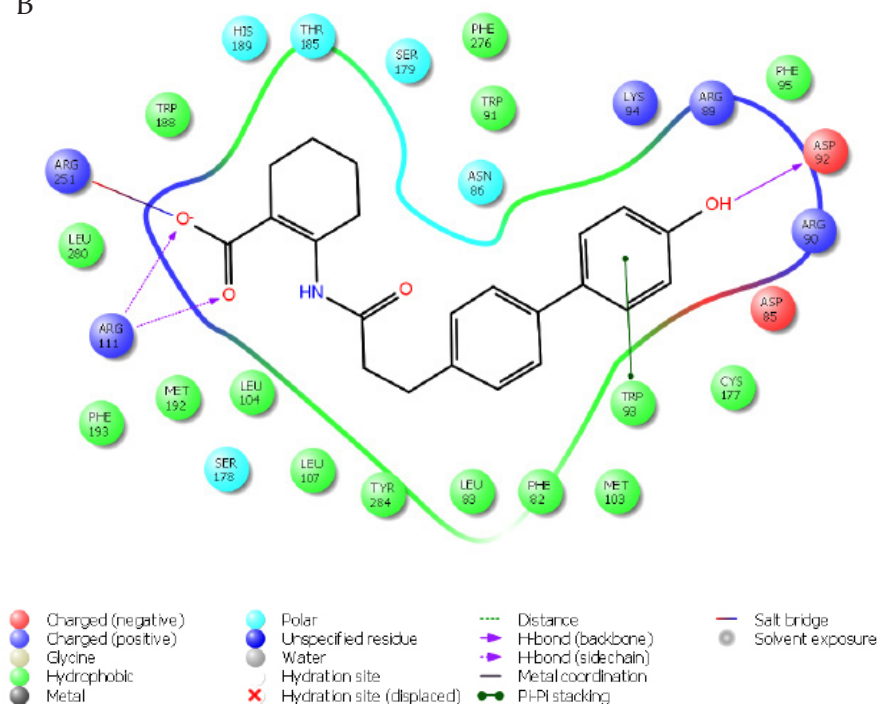
Fig. 3. Interaction map of 6g (A) and 6z (B) with surrounding residues in a composite homology model of HCA 2 receptor was constructed based on the structure of both the Serotonin 2b receptor co-crystallized with ergotamine (Protein Data Bank: 4IB4) and the crystal structure of the Free Fatty Acid receptor 1 bound to TAK-875 (Protein Data Bank: 4PHU) [15, 16] .
