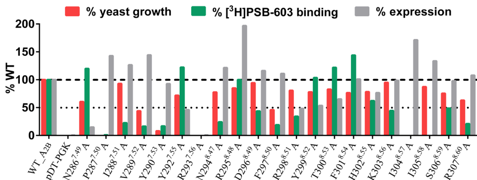
Fig. 2. Characterization of the NPxxY motif and helix 8 mutants of the adenosine hA 2B receptor in the strain MMY24 (G α13 ): agonist efficacy (■), antagonist binding (■), and expression level (■).
