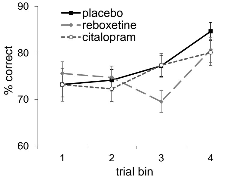
Supplemental Figure 1. Learning curves illustrating the change in tone discrimination performance over the four consecutive trial bins in the diminishing-utility task, separately for each treatment group (error bars indicate standard errors of the mean).
