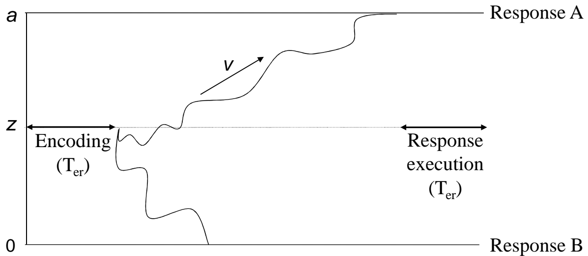
Figure 1. An illustration of the diffusion model. The parameters are: a = boundary separation, z = starting point, v = drift rate, T_{er} = mean nonddecision time. The sample paths represent moment-by-moment fluctuations in the evidence favoring the two possible responses, which is due to noise in the decision process. The decision process starts at z and terminates when one of the two boundaries is reached. The duration of T_{er} determines the additional time needed for stimulus encoding and response execution.
