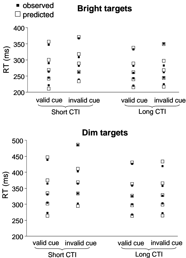
Figure 7. The observed and predicted .1, .3, .5, .7 and .9 quantile RTs in Experiment 2 as a function of target brightness (bright, dim), cue-target interval (CTI) and cue validity.
