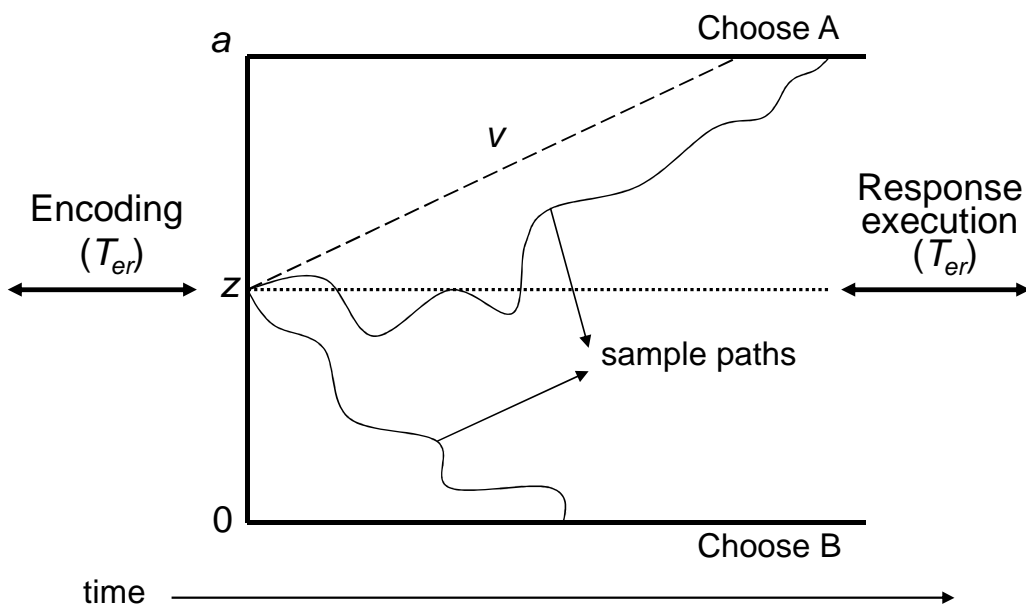
Figure 4. An illustration of the diffusion model. The parameters are: a = boundary separation, z = starting point, v = drift rate, T_{er} = mean nonddecision time. The sample paths represent moment-by-moment fluctuations in the evidence favoring the two possible responses, which is due to noise in the decision process. The decision process starts at z and terminates when one of the two boundaries is reached. The duration of T_{er} determines the additional time needed for stimulus encoding and response execution.
