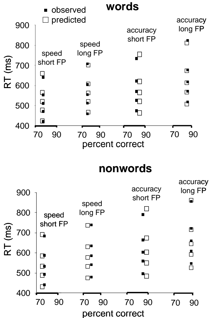
Figure 3. The observed and predicted (by T_{er} model) .1, .3, .5, .7 and .9 correct quantile RTs in Experiment 1, plotted against the corresponding proportions correct, as a function of word type, instruction (speed/accuracy) and foreperiod duration.
