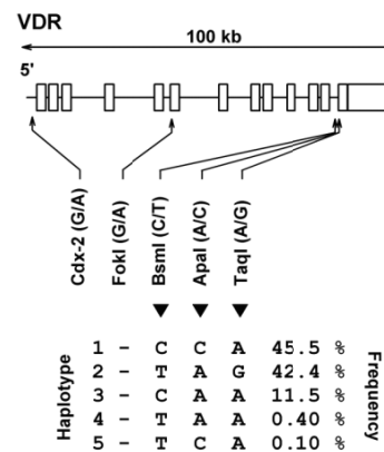
Figure 3.1. The VDR gene structure and haplotypes. The VDR gene spans a genomic region of 100 kb and contains 14 exons (indicated with boxes). The approximate positions of the five polymorphisms analyzed in this study are indicated with arrows. The BsmI , Apal and TaqI polymorphisms are in strong linkage disequilibrium (LD) and define five haplotypes. The first three haplotypes, haplotype 1, haplotype 2 and haplotype 3 have previously been described as baT, BAt and bAT, respectively.
