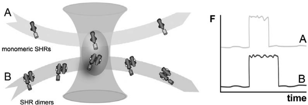
Figure 5. Fluorescence Correlation Spectroscopy (FCS). By using the microscope objective lens to focus the laser beam, a diffraction limited excitation volume is created. The emitted fluorescence signal (F) from this observation volume fluctuates as labeled molecules diffuse in and out, and the duration of the fluctuations are related to the average time individual models reside within the volume. One such an event is depicted in the graph. The residence time can be used to determine the diffusion coefficient for the fluorescent molecules, which is dependent on their size and interaction with other proteins. For example, it can be used to discriminate monomeric Steroid Hormone Receptors (SHRs, A) from dimeric complexes (B).
