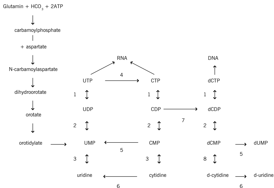
Figure 1 Pyrimidine synthesis
