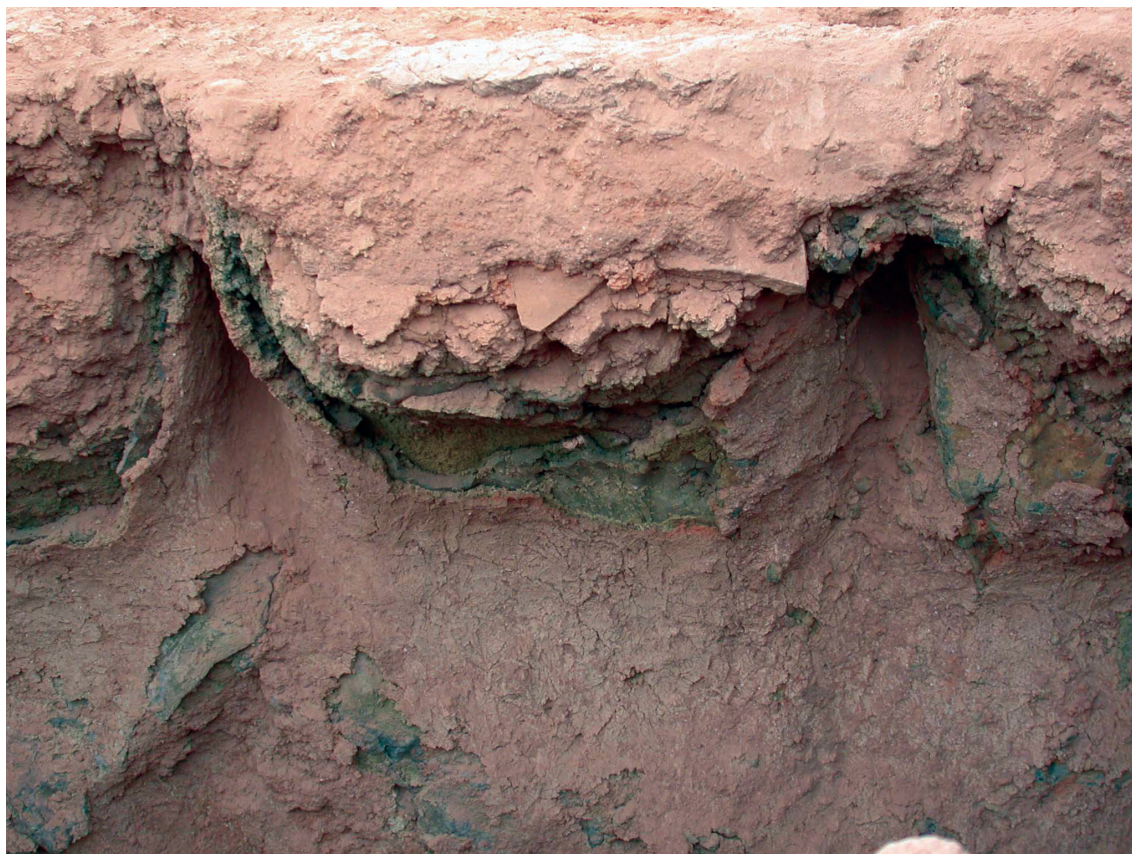
Fig. C.6: Kiln Q, the plaster on the inside of the fire chamber and the flue holes. The highly burnt bright green plaster has been re-applied a number of times. Sherds were used to fill gaps in the mud-brick arches.
