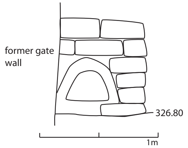
Fig. C.23: Kiln CJ/V in square K8, front view of fueling hole (view B, looking south)
