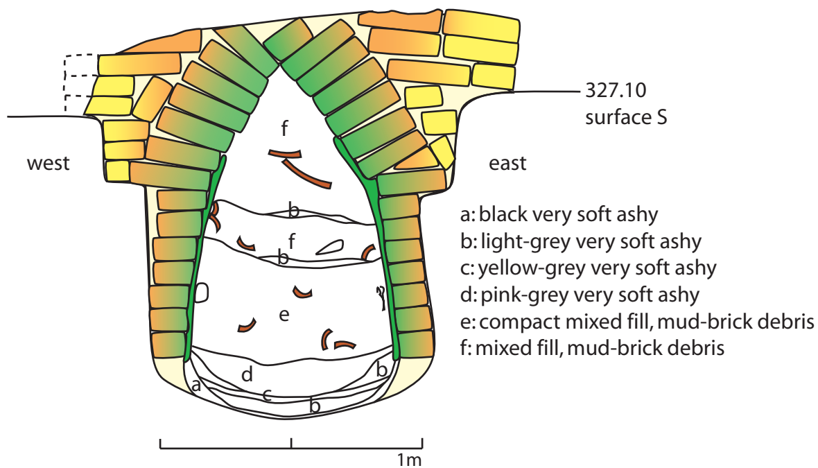
Fig. C.28: Kiln K in square J7, section B, looking north.
