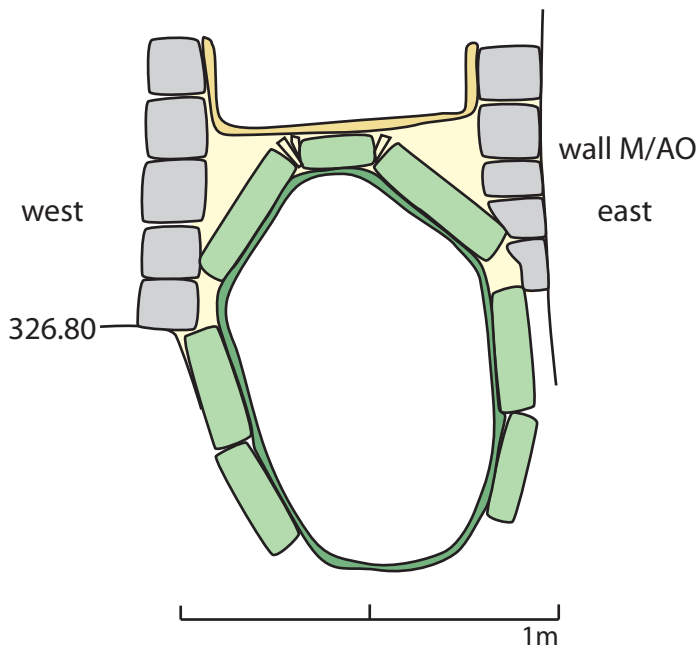
Fig. C.22: Kiln CJ/V in square K8, section E-W (A).
