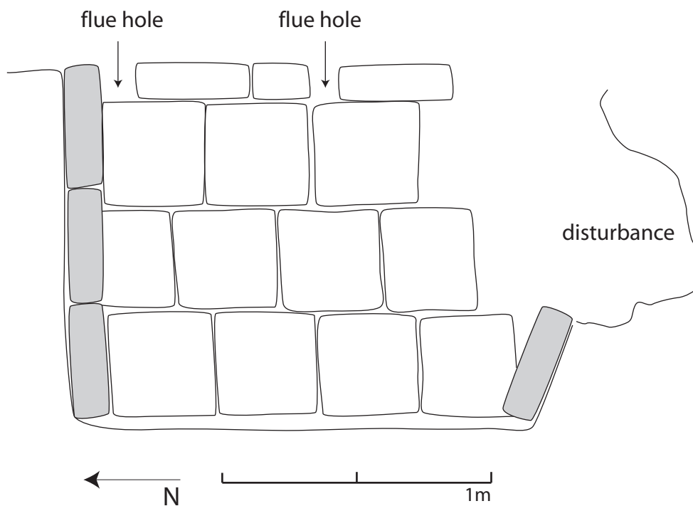
Fig. C.10: Kiln L in square N12, section (N-S).
