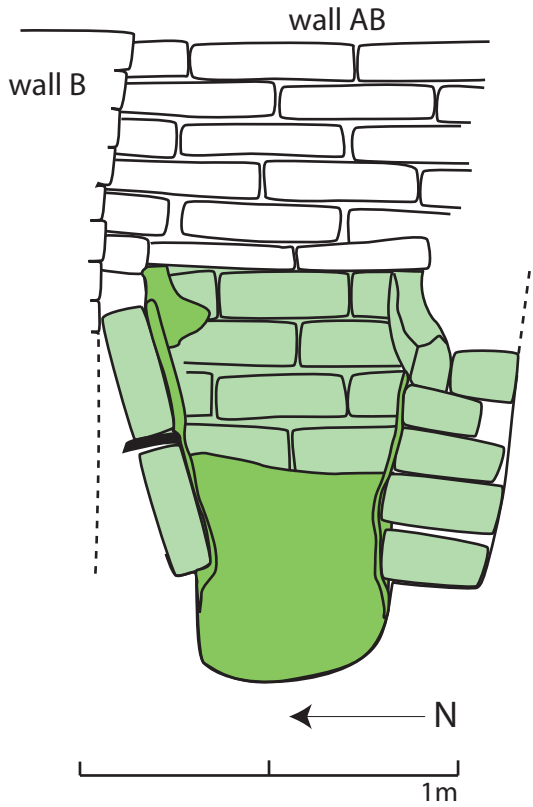
Fig. C.14: Kiln H/AE in square H8, section A.
