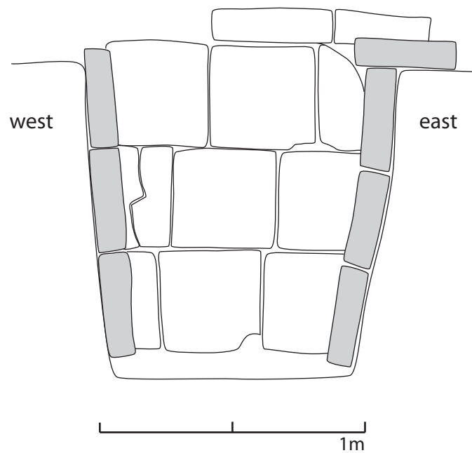
Fig. C.9: Kiln L in square N12, section (E-W).
