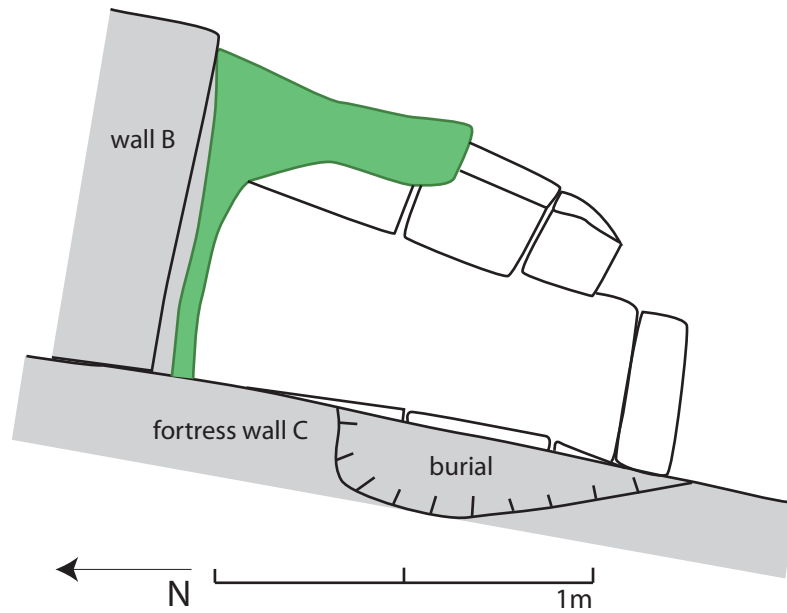
Fig. C.18: Kiln I in square H8 (level 5), top plan.
