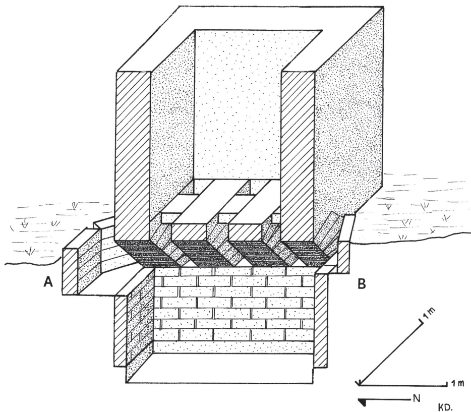
Fig. C.29: Kiln K in square J7, reconstruction drawing.
