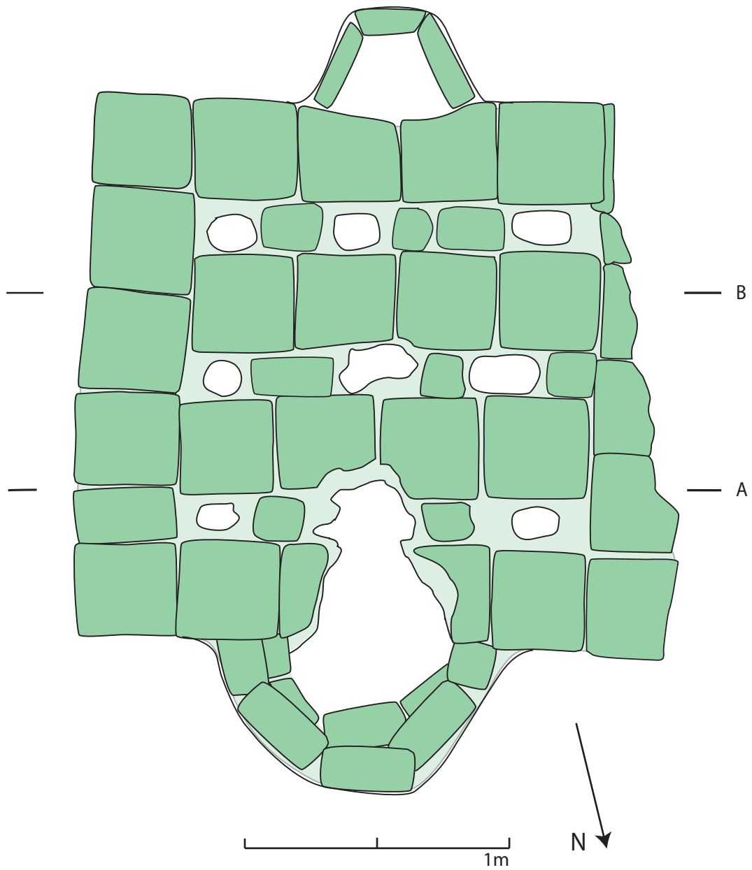
Fig. C.26: Kiln K in square J7 (level 4), schematical top plan.
