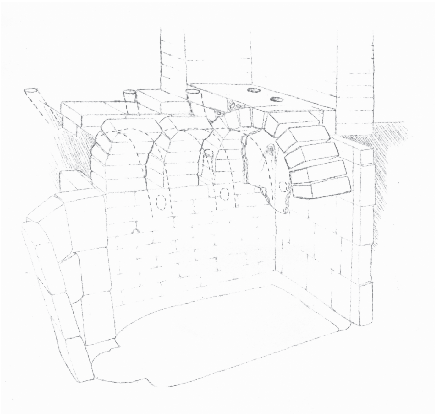
Fig. C.3: Kiln Q in square N11, reconstruction drawing.
