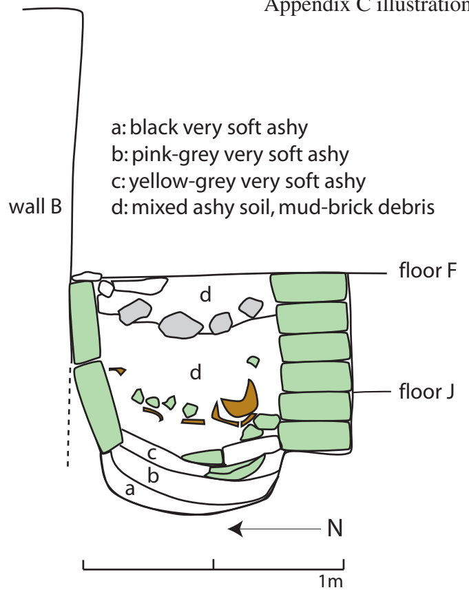
Fig. C.15: Kiln H/AE in square H8, section B: section through the kiln fill.
