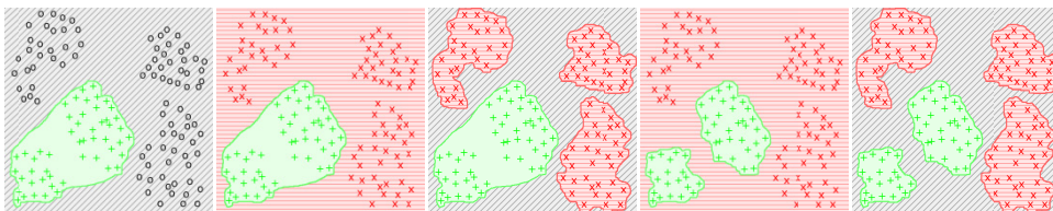
Figure 2.4: Illustration of several classification variations (from left to right): one-class, two-class, 1+x , x+1 , x+y . In the figures the green pluses refer to positive examples, the red crosses to negative examples and the black circles to neutral examples. The light green area is then classified as positive, the horizontally striped light red area as negative and the diagonally striped gray area as neutral.
