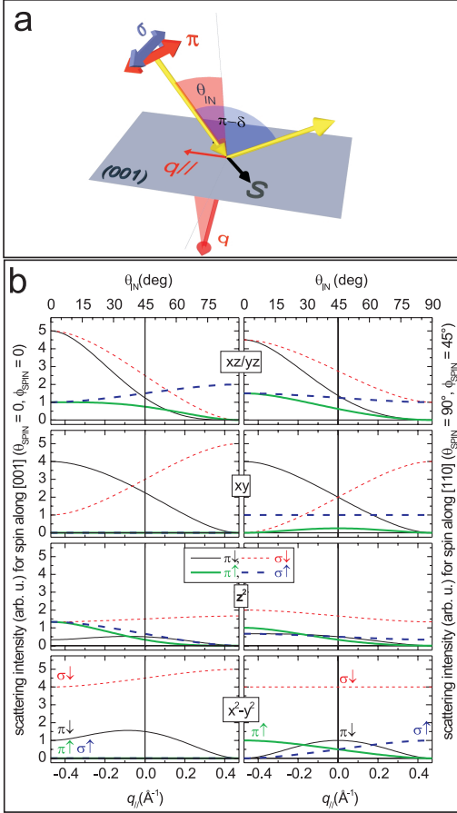
Figure 4.10: L_3 RIXS cross section for a single \text{Cu}^{2+} ion with \sigma and \pi polarization of the incident beam. (a) The geometry: the scattering plane is (100), scattering angle 90^\circ , the incident photons impinge at an angle \theta_{IN} to the [001] direction ( c axis). (b) Scattering intensities to different orbital and spin orientations, starting from a (x^2-y^2)_{\downarrow z} state (left panels) and a (x^2-y^2)_{\downarrow xy} groundstate (right panels) as a function of \theta_{IN} or alternatively the in-plane transferred momentum q_{||} . For \downarrow_z , i.e. , spin along [001], the spin flip cross section vanishes (bottom left), not so for \downarrow_{xy} , with spin along [110] (right).
