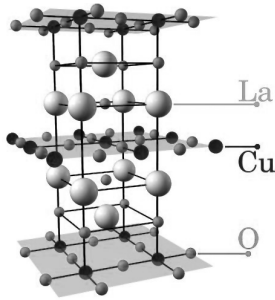
Figure 4.1: The crystal structure of \text{La}_2\text{CuO}_4 . The \text{CuO}_2 layers are separated by electronically inactive \text{LaO} layers. Figure by M. Berciu.
