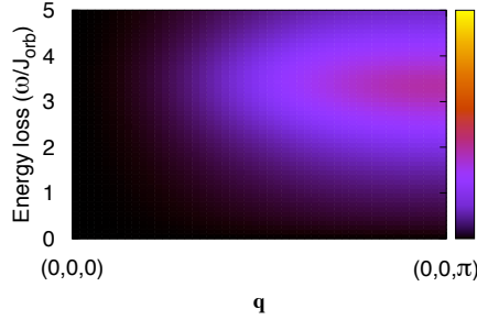
Figure 5.12: RIXS spectrum for two-site processes within the superexchange model. The color scale denotes the intensity. The figure shows \mathbf{q} running from (0,0,0) to (0,0,\pi) . One-orbital creation is not allowed for the superexchange modulation mechanism. The intrinsic energy broadening \gamma of the orbitalon states is \gamma = 0.4 J_{\text{orb}} \approx 30 meV, and the added experimental resolution of 27.5 meV [202] is approximately 0.34 J_{\text{orb}} .
