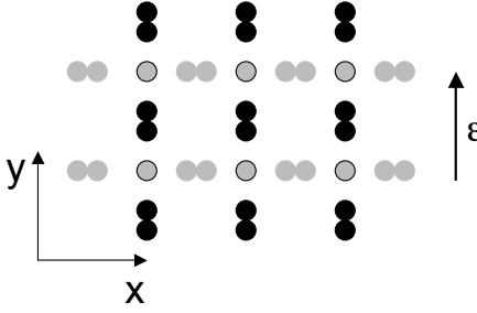
Figure 4.17: Polarization dependence of the absorption of X-rays at the O K edge. The oxygen ions with the black 2p orbitals can be excited with RIXS when the polarization is directed along the y axis, while the gray oxygen ions are then inactive. The gray circles with black borders represent the Cu ions.
