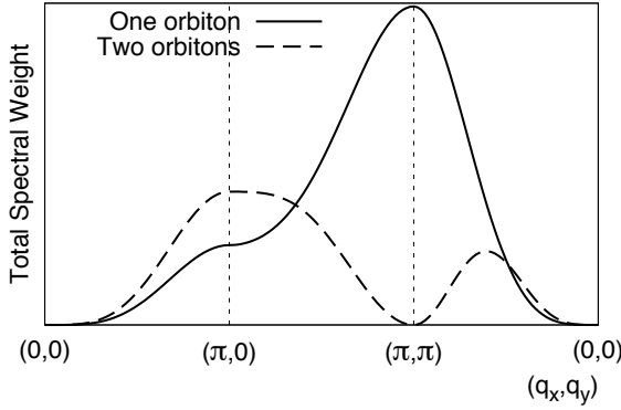
Figure 5.5: Comparison of the energy integrated spectral weight of the one- and two-orbital RIXS spectra at fixed momentum transfer \mathbf{q} .
