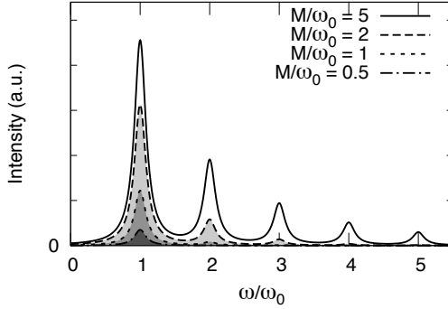
Figure 7.1: RIXS phonon cross section for Einstein phonons with energy \omega_0 , for different electron-phonon couplings M . We take \Gamma/\omega_0 = 5 (a typical value at the copper L edge), and an incident energy corresponding to the maximum in the XAS signal. The polarization dependence is omitted in this plot, as well as the zero loss peak, which shifts to the Bragg peaks in an ideal crystal.
