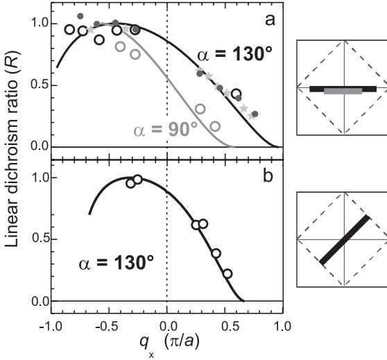
Figure 4.15: Single magnon spectral weight measured at the copper L_3 edge of various cuprates with transferred momentum along (a) the [100] direction, and (b) the [110] direction. The open circles refer to \text{La}_2\text{CuO}_4 , the filled circles to (\text{Sr,Ca})\text{CuO}_2 (prepared as a thin film on \text{SrTiO}_3 ), and the stars to strongly underdoped \text{NdBa}_2\text{Cu}_3\text{O}_{6+\delta} . The data were taken at T = 15 K. \alpha is the scattering angle. Figures from Ref. [21].
