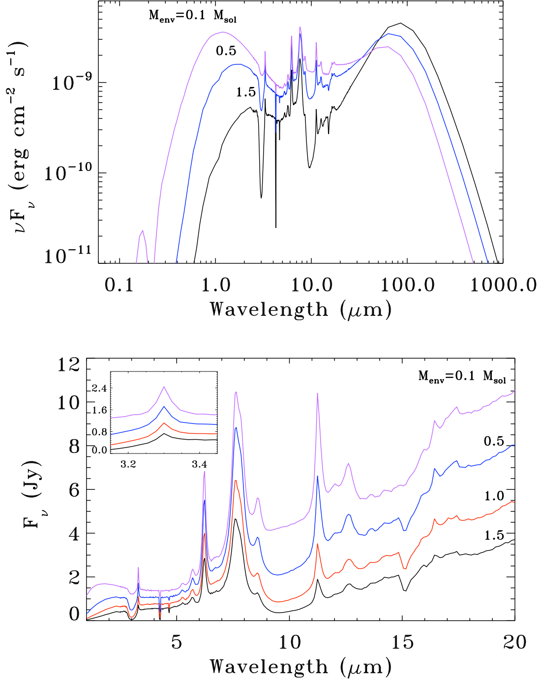
Figure 5.6: Model SED (top) and blow-up of spectrum (bottom) with M_{\text{env}} = 1.5 (black), 1.0 (red), 0.5 (blue) and 0.1 (purple) M_\odot at i = 45^\circ . The curve for 1.0 M_\odot was omitted from the SED plot for clarity. The inset shows a blow-up of the 3.3 μm PAH feature.
