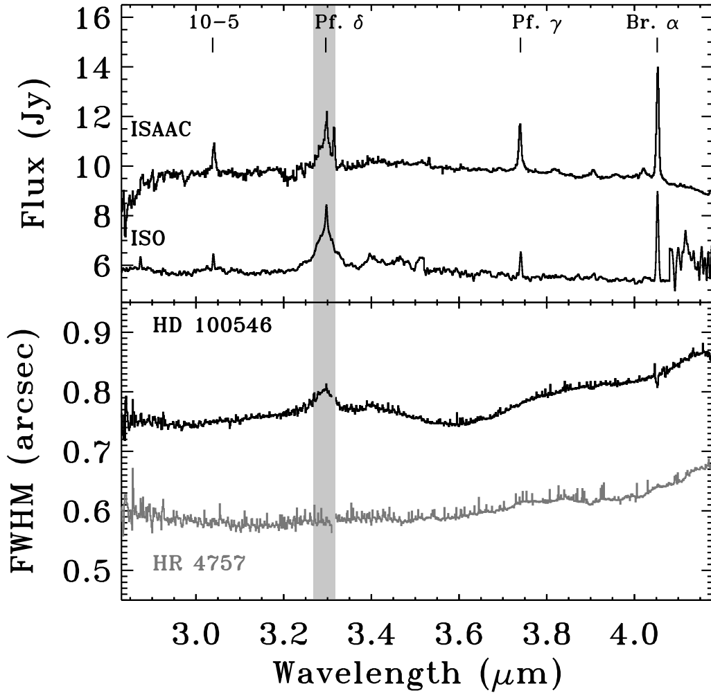
Figure 4.5: ( Upper panel ) ISAAC L-band spectrum of HD 100546, scaled by a factor 1.25 to match the ISO spectrum and then shifted by +4 Jy for clarity. The grey band highlights the position and FWHM of the 3.3 \mu\text{m} PAH feature as determined in this paper. ( Lower panel ) FWHM of the spatial profile, as extracted from 2D spectral image, of HD 100546 ( black line ) and its corresponding standard HR 4757 ( grey line ). The FWHM of the latter agrees with that of the HD 100546 continuum after correction for airmass and seeing differences.
