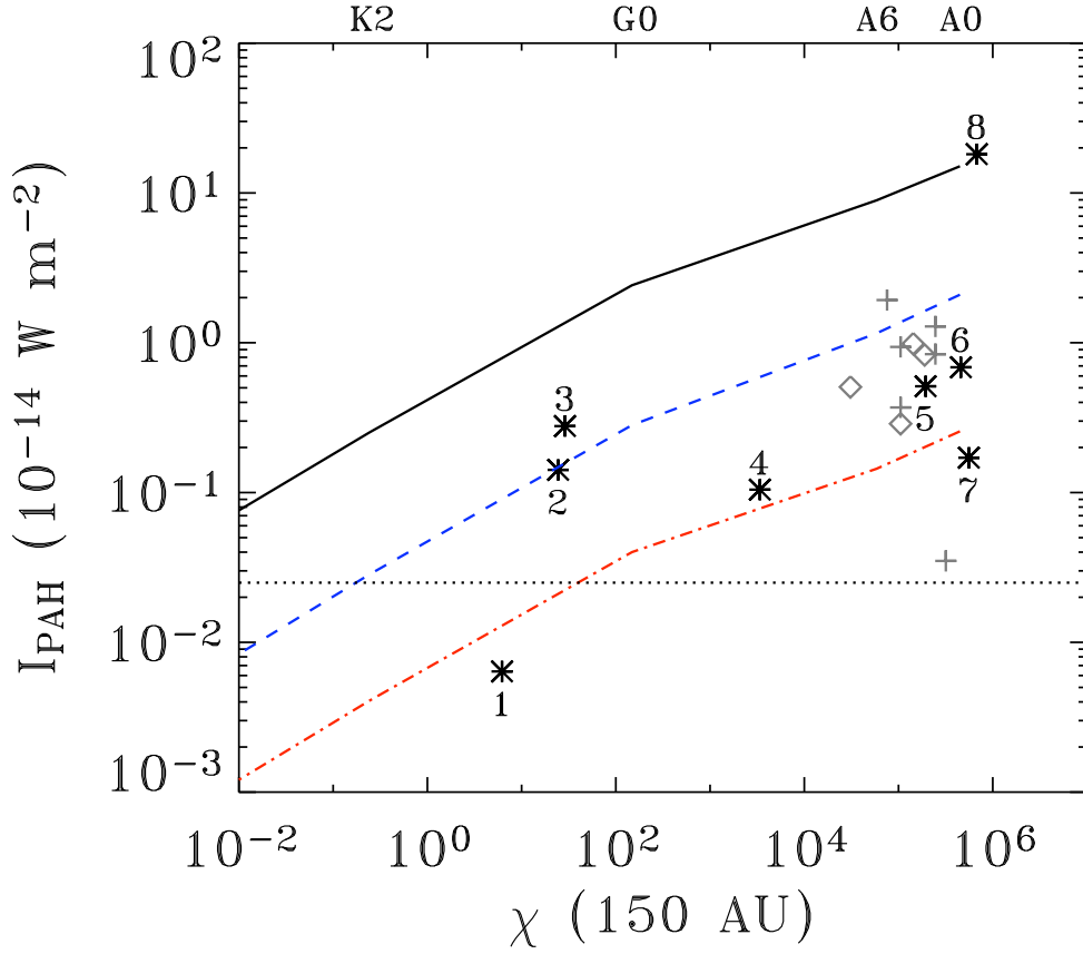
Figure 2.14: Strength of 11.2 \mu\text{m} PAH feature I_{\text{PAH}} (scaled to a distance of 150 pc) versus \chi , the integrated FUV field (6–13.6 eV) for a ZAMS star, after Habart et al. (2004, their Figure 8). Solid line represents our template model, based on Fig. 2.9; dashed and dash-dotted lines represent our models with a 10x and 100x lower PAH abundance respectively. Black ‘*’ symbols are for c2d sources. Grey diamonds are ISO upper limits of the 11.2 \mu\text{m} feature strength for Herbig Ae sources, grey ‘+’ symbols are ISO detections. c2d sources are labelled as follows. 1: T Cha; 2: LkH \alpha 330; 3: SR 21 N; 4: HD 135344; 5: RR Tau; 6: VV Ser; 7: HD 101412; 8: HD 98922. The dotted grey line indicates our typical 3\sigma sensitivity limit of 2.5 \times 10^{-16} \text{ W m}^{-2} for sources at d = 150 \text{ pc} .
