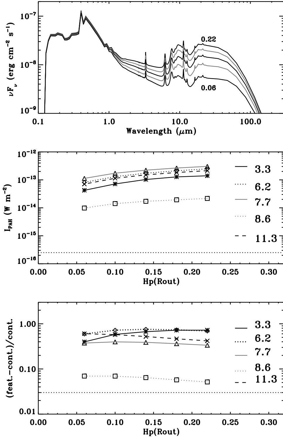
Figure 2.13: Top panel: Model SEDs of a star+disk with PAH, with scale height of outer disk H/R_{\text{out}} = 0.06, 0.1, 0.14, 0.18 and 0.22 at a distance of 150 \text{ pc} . Middle panel: PAH line fluxes for the corresponding models. Bottom panel: Feature to continuum ratio of the various features. The dotted line indicates our observational limits.
