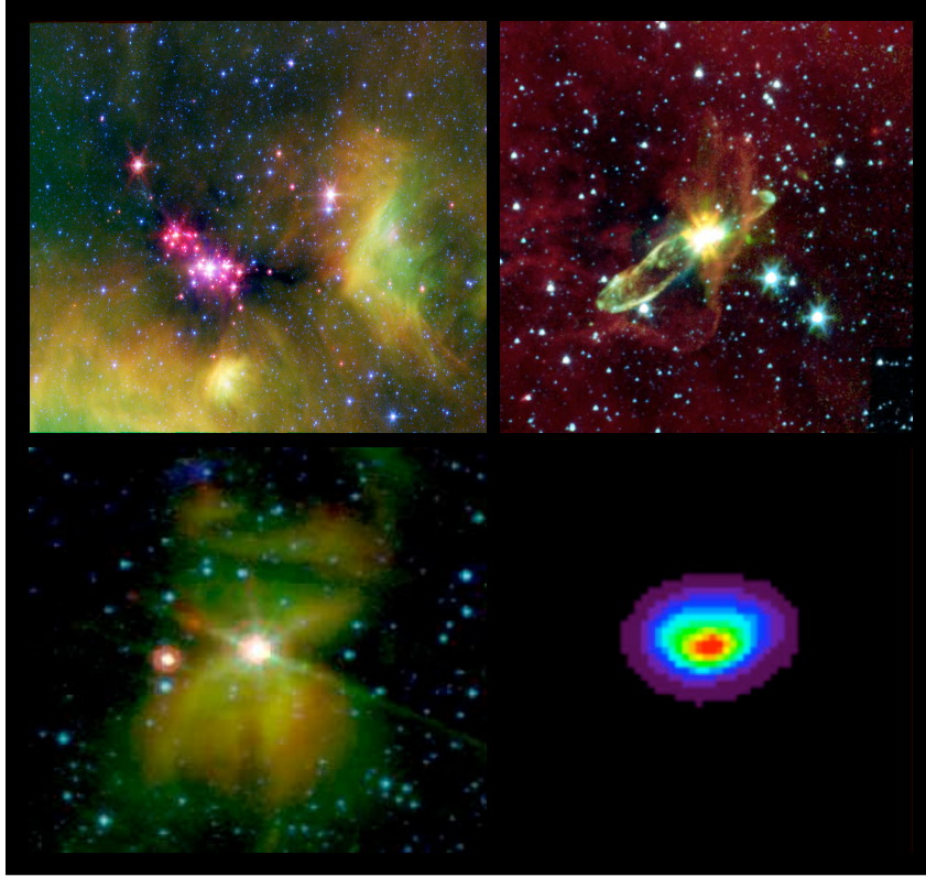
Figure 1.4: PAH emission observed toward a variety of astrophysical environments: diffuse interstellar dust in the Serpens star-forming region (PAH 8\ \mu\text{m} indicated in green, top-left, \sim 2\ \text{pc} on the side), molecular cloud with embedded object HH 46 and outflows (PAH 8\ \mu\text{m} indicated in red, top-right, 0.7\ \text{pc} on the side), VV-Ser, young star with disk in remnant cloud (bottom-left, 5 \times 10^4\ \text{AU} on the side), close-up of circumstellar disk around IRS 48 at 11.25\ \mu\text{m} (bottom-right, 600\ \text{AU} on the side). Data in the first three panels all come from the c2d Spitzer Legacy program, the IRS 48 image is taken with VLT-VISIR.
