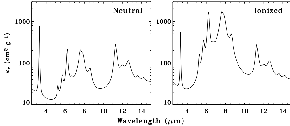
Figure 1.3: PAH opacities of neutral (left) and single ionized (right) C_{100}H_{24} , based on Draine & Li (2007) and Mattiotta et al. (2005). Note the order of magnitude enhancement of the 6.2, 7.7 and 8.6 \mu m features for the ionized species.
