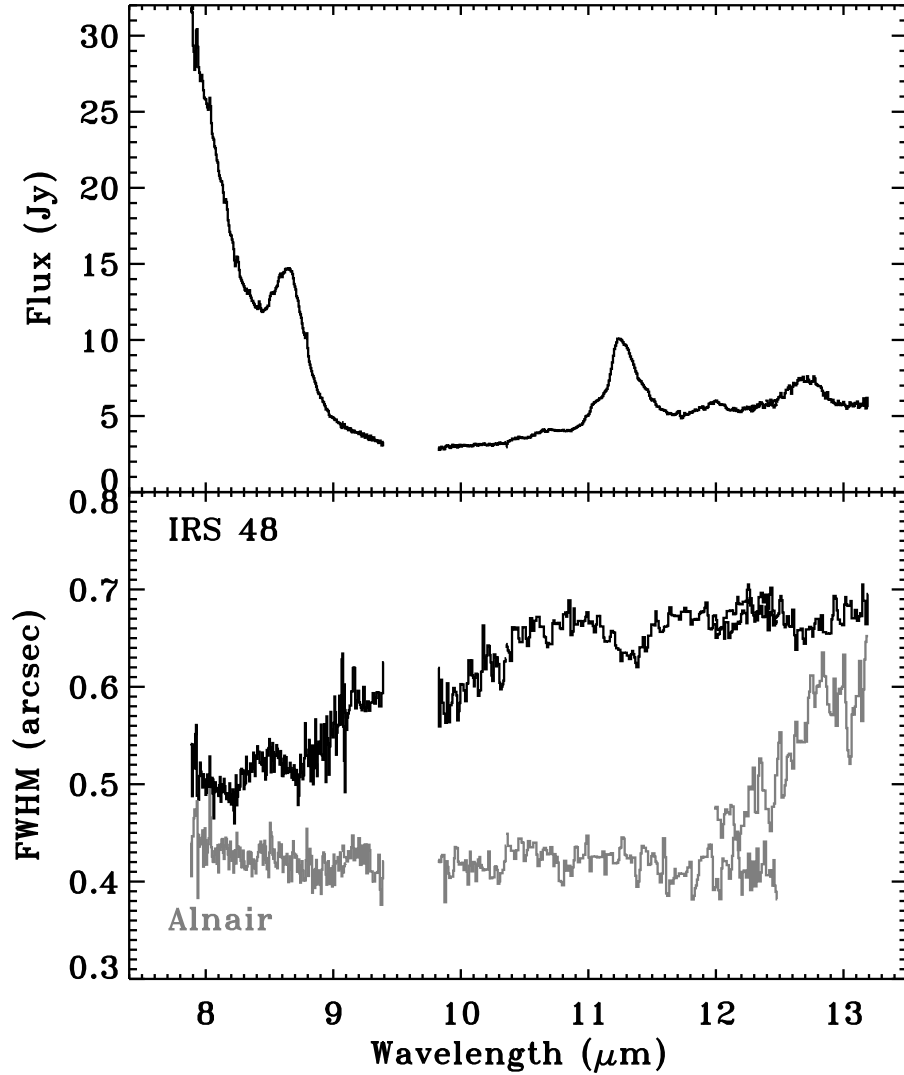
Figure 4.13: (Upper panel) VISIR N-band spectrum of IRS 48. (Lower panel) FWHM of spatial profile of IRS 48 and standard star Alnair.
