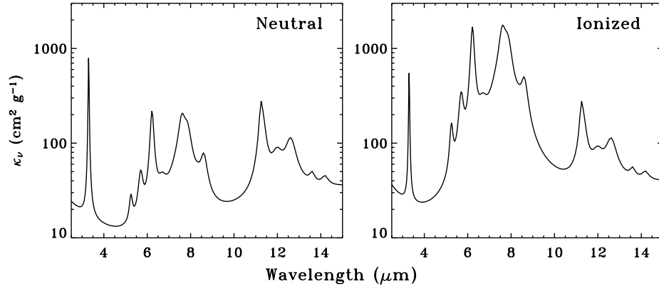
Figure 1.3: PAH opacities of neutral (left) and single ionized (right) C_{100}H_{24} , based on Draine & Li (2007) and Mattioda et al. (2005). Note the order of magnitude enhancement of the 6.2, 7.7 and 8.6 \mu m features for the ionized species.
