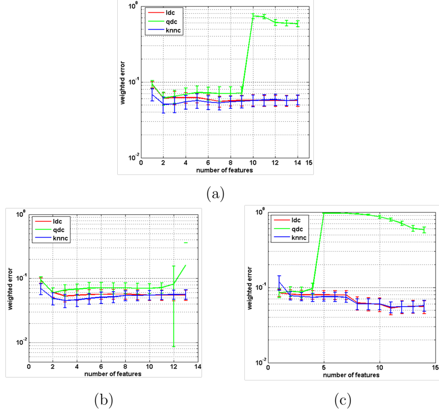
Figure 2.5. Weighted classification error curves, with (a) Individual feature selection, (b) Branch and bound feature selection and (c) Backward feature selection.
