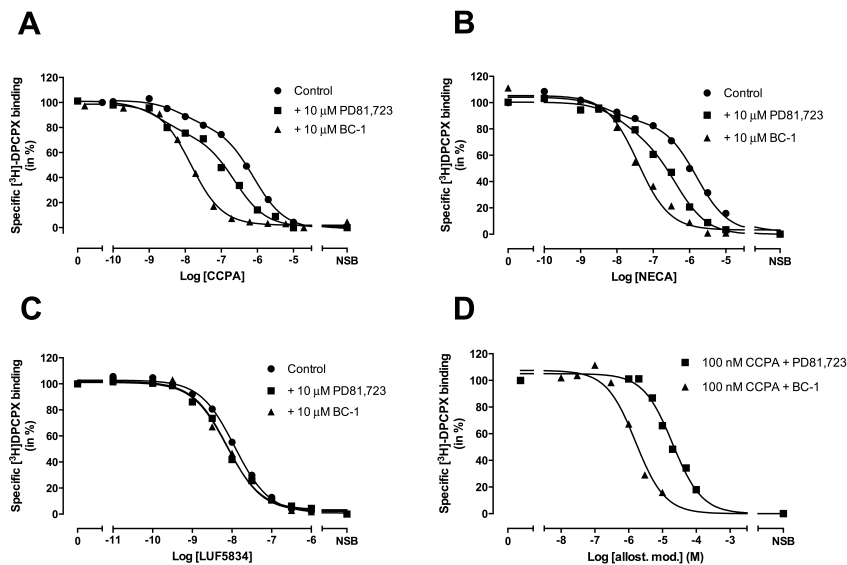
Figure 6.3 | Displacement of specific [^3\text{H}]\text{-DPCPX} binding from the adenosine A_1 receptor at 25 °C by CCPA (Panel A), NECA (Panel B) or LUF5834 (Panel C) in the absence or presence of 10 \mu\text{M} PD81,723 or BC-1 or by 100 nM CCPA (normalized as 100%) in the presence of increased concentrations of PD81,723 or BC-1 (Panel D). Representative graphs from one experiment performed in duplicate.
