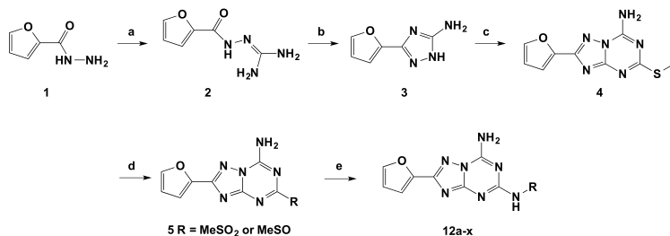
Scheme 4.1 | General synthesis route to 24 triazolotriazine derivatives. Reagents and conditions: (a) S-methylisothiurea sulfate (2:1), 4 % NaOH (aq) RT; (b) H 2 O, RT; (c) (1) (MeS) 2 C=NCN, heat, 180 °C, (2) CH 2 Cl 2 -CH 3 OH (2:1), reflux; (d) mCPBA (70 % strength), CH 2 Cl 2 , 0 °C-> RT; (e) (Et) 3 N, CH 3 CN.
