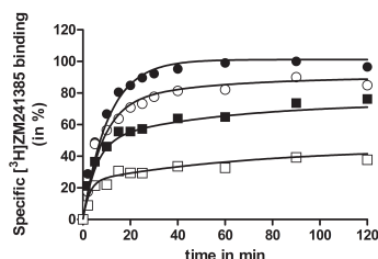
Figure 5.5 | Competition association experiment with [ ^3\text{H} ]-ZM241385 in the absence of ligand (solid spheres) or in the presence of one-fold K_i value (empty spheres), three-fold K_i value (solid squares) or ten-fold K_i value (empty squares) of unlabeled ZM241385. Representative graphs from one experiment performed in duplicate (see Table 5.1 for kinetic values).
