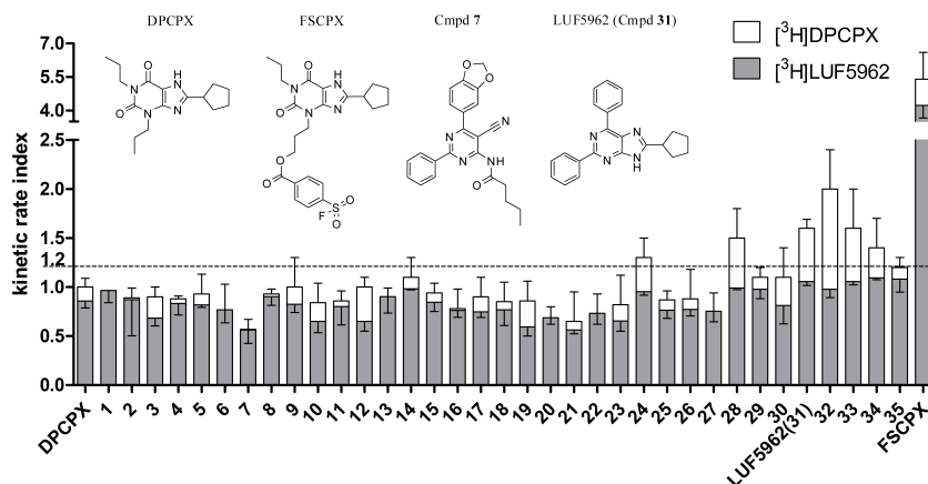
Figure 3.5 | Kinetic rate indexes (KRI) of 35 in-house hA_1R antagonists, DPCPX and FSCPX. 16–18 The KRI values of the same panel of unlabeled ligands against [^3H] -LUF5962 (gray bars) are integrated with the results obtained with [^3H] -DPCPX (white bars). Values were obtained from the dual-point assays and calculated by using Equation 6. The KRI of the reference compounds, unlabeled DPCPX or LUF5962 (compound 31 ), were determined approximately 1.0 in the respective screen. FSCPX was the ‘tool compound’ and known to bind irreversibly to hA_1R . Seven compounds with a kinetic rate index \geq 1.2 (the stippled line) were found using [^3H] -DPCPX and no compounds with a kinetic rate index \geq 1.2 were found using [^3H] -LUF5962 (excluding FSCPX in both cases). Data are shown as mean \pm s.e.m from three separate experiments each performed in duplicate. Chemical structures of DPCPX, FSCPX, compound 7 and LUF5962 (compound 31 ) are also presented.
