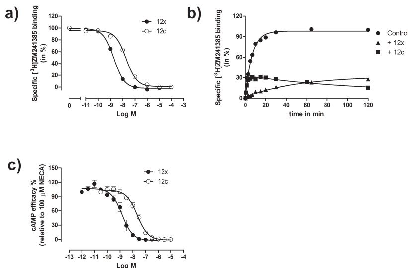
Figure 4.2 | (a) Displacement of specific [ ^3H ]-ZM241385 binding from the hA_{2A} receptor by two representative compounds, namely 12x and 12c ; (b) [ ^3H ]-ZM241385 competition association binding in the absence of ligand (control) and in the presence of 10 \times K_i of unlabeled 12x or 12c . Data was fitted to the equation described in the experimental section to calculate k_{on} and k_{off} of unlabeled ligands. Representative graphs from one experiment performed in duplicate (See Table 4.1 and 4.2 for affinity and kinetic values); (c) Concentration-effect curves for 12x and 12c in a cAMP assay. Data were obtained by adding HEK293 hA_{2A} R cells to the mixture of the antagonist ( 12x or 12c ) and 100 nM NECA for an incubation of 30 min. Data are expressed as mean \pm s.e.m from at least three independent experiments. (See Table 4.3 for potency values).
