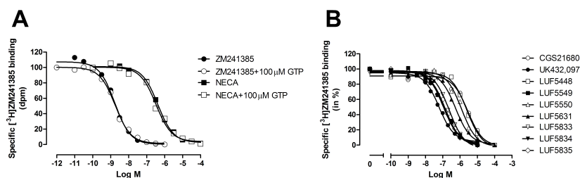
Figure 5.3 | Panel A: displacement of specific [^3\text{H}]\text{-ZM241385} binding from the \text{hA}_{2\text{A}}\text{R} by ZM241385 and NECA in the absence (closed symbols) or presence of 100 \mu\text{M} GTP (open symbols). Panel B: displacement of specific [^3\text{H}]\text{-ZM241385} binding from the \text{hA}_{2\text{A}}\text{R} by the other nine agonists. Representative graphs from one experiment performed in duplicate.
