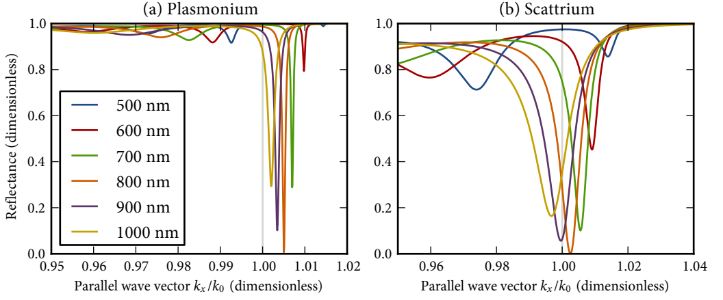
Figure 5.14: SPR curves for a number of representative wavelengths, for an Otto experiment with (a) plasmonium separated from a n = 1.5 glass-like substrate by a vacuum gap of 2.4\ \mu\text{m} ; (b) scattrium separated from the same substrate, by a vacuum gap of 1.4\ \mu\text{m} . The gaps' thicknesses are designed for critical coupling at \lambda = 800\ \text{nm} , but not for other wavelengths. Compare to Fig. 5.11.
