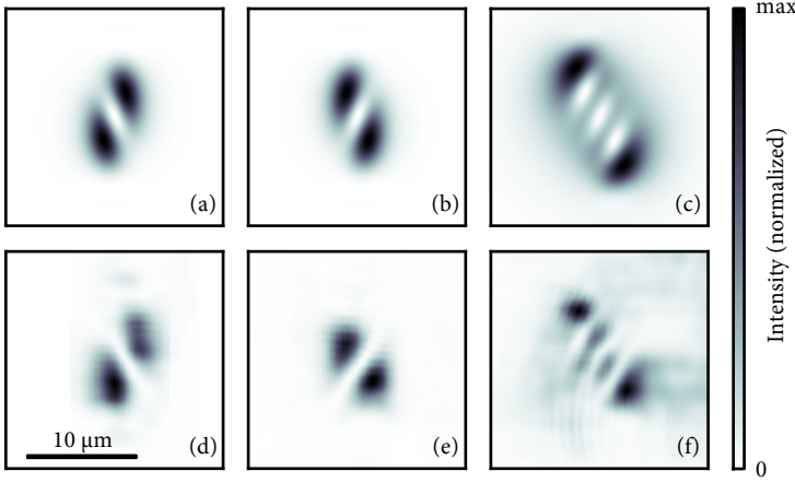
Figure 4.5: Calculated (a–c) and experimental tomograms (d–f) for beams on slits separated by 25\text{ }\mu\text{m} , with vortex charge Q = +1 (a and d), Q = -1 (b and e), and Q = -3 (c and f). Note that the intensity zeroes in (c) and (f) occur nicely along a straight line.
