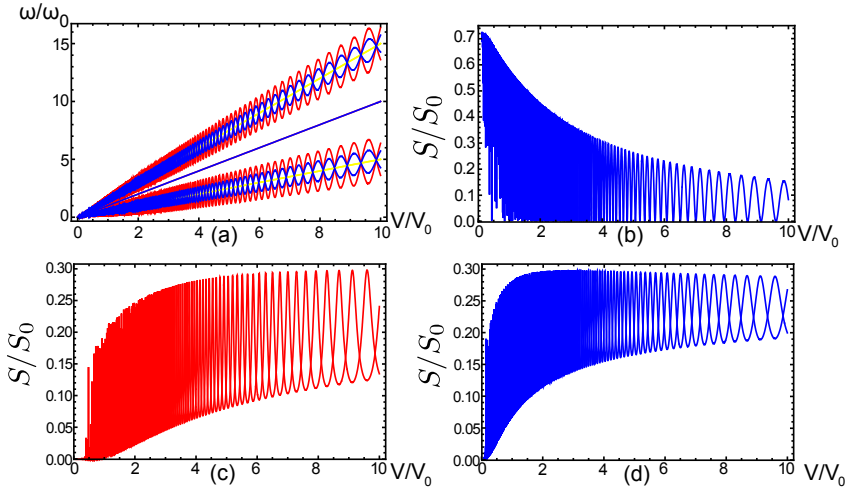
Figure 5.6. The generic case of parity separation. Here, V_0 = 4\pi G_0^2/\bar{\epsilon} , \omega_0 = 2eV_0/\hbar , \bar{\epsilon}/\omega_0 = 30 , S_0 \equiv I_m^2/2 . a. Peak positions. Four distinct noise peaks converge to half-integer multiples of \omega_j upon increasing voltage. b. Spectral intensity of the main peak at \omega_j . It is contributed by both parities. c. The same for the first two even parity peaks. d. The same for the two odd parity peaks.
