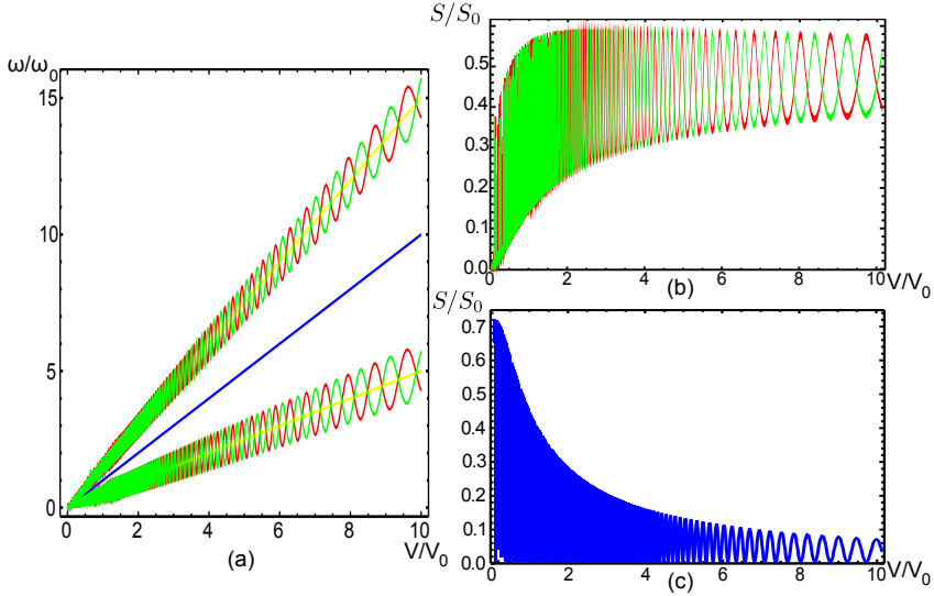
Figure 5.4. The slow decoherence limit. We chose \tilde{\epsilon}/eV_0 = 30 for all plots. (a). Frequency positions of the noise peaks versus V ( \omega_0 = (2e/\hbar)V_0 ). The main ones are at n\omega_j while the positions of additional peaks oscillate converging at (n + 1/2)\omega_j . Only n = 0, 1 are shown. (b) Integrated noise intensity (in units of S_0 \equiv I_m^2/2 ) of the first two additional peaks. (c) The same for the n = 1 main peak.
