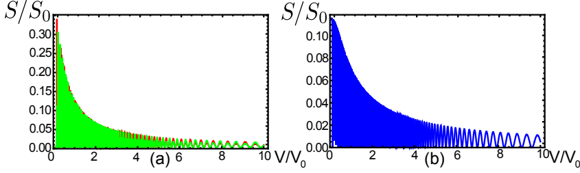
Figure 5.5. Intensities of the high-frequency noise peaks. The parameters are the same as in Fig. 4 of the main text. Left: two additional peaks with frequencies converging to (3/2)\omega_j at V \gg V_0 . Right: main peak at 2\omega_j .
