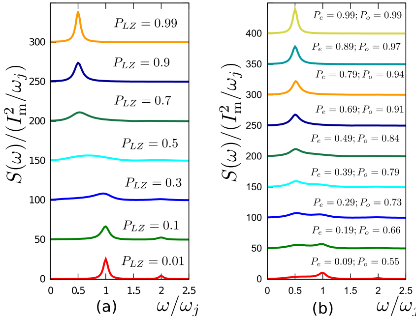
Figure 5.3. The spectral intensity S(\omega) of the current noise for a set of V corresponding to LZ probabilities shown, in the limit of fast decoherence. a. Indistinguishable parities P_e = P_o = P_{LZ} ; b. P_e \neq P_o ( G_e = 4G_o ). Distinct peaks at multiples of \omega_j at P \ll 1 transmute into a single peak at \omega_j/2 at P \approx 1 . ( \Gamma_r = \Gamma_q = 0.02\omega_j for all plots).
