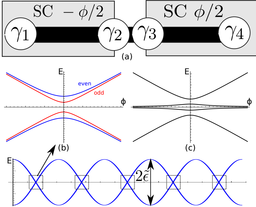
Figure 5.1. a. A Majorana Josephson junction is formed by mounting a nanowire (black) on two superconducting leads (grey) resulting in four Majoranas \gamma_{1-4} . b. The energies of the many-body junction states versus phase near an avoided crossing point. c. Corresponding Andreev levels. d. The energies of the junction states versus phase at a bigger scale. Far from the avoided crossing points, the energies of even and odd states are indistinguishably close. This corresponds to two zero-energy Andreev levels.
