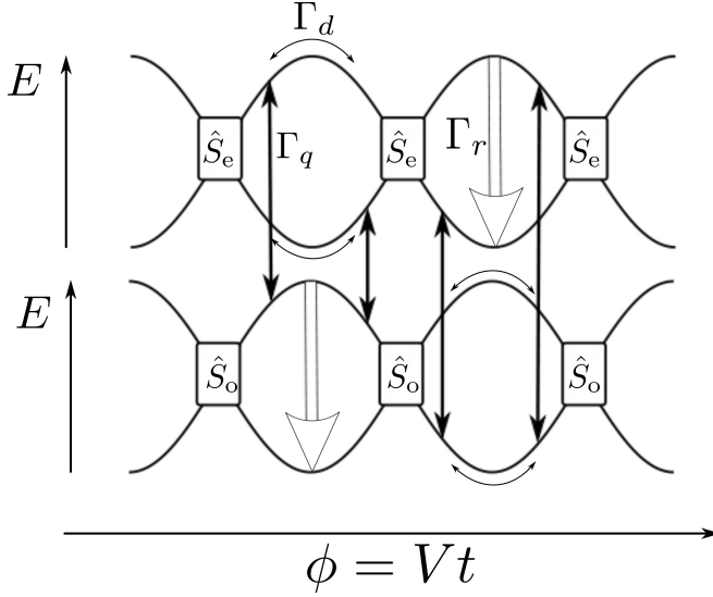
Figure 5.2. Processes affecting the junction dynamics. In between the parity-dependent Landau-Zener scatterings (described by 2 \times 2 matrices \hat{S}_{o,e} ) the junction is subject to dephasing (with a rate \Gamma_d ), relaxation ( \Gamma_r ) and quasiparticle poisoning ( \Gamma_q ).
