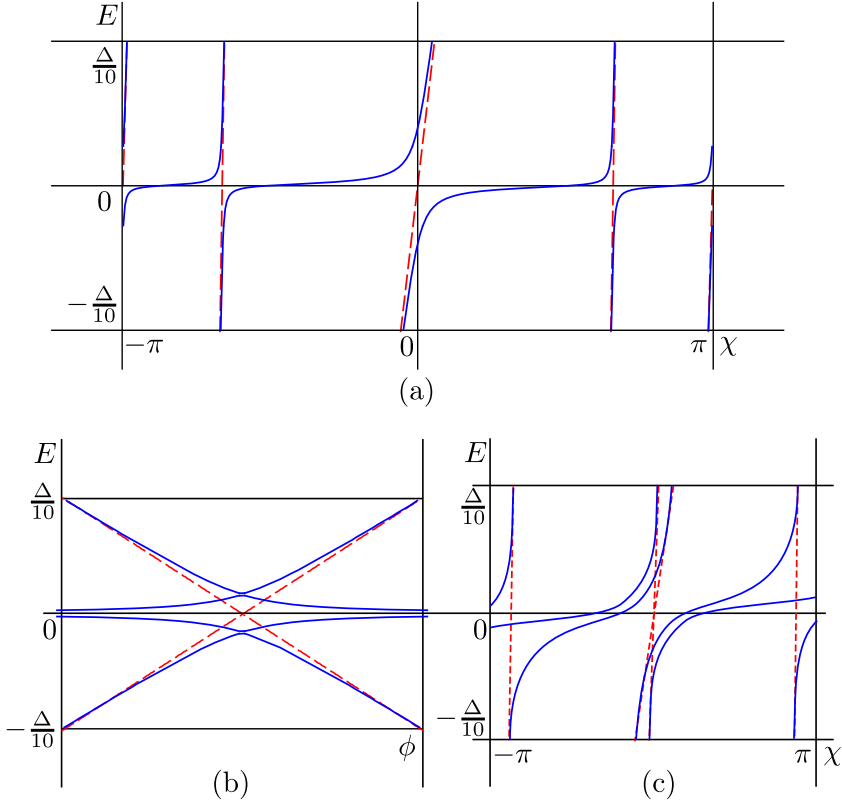
Figure 2.4. (a): Energy dependence of eigenvalues for NS junction in a narrow energy interval illustrates the topological triviality of s -matrix for finite length of the contact ( L=7 in units of [8]). Dashed lines: "high"-energy TNTM eigenvalues. We see the reconnection of neighboring eigenvalues. (b): Andreev levels in SS junction versus superconducting phase difference at L_1 = L_2 = 7 (solid lines) as compared to TNTT case at L_{1,2} = \infty (dashed lines). (c) Energy dependence of eigenvalues for case (b) and \phi = \pi . Dashed lines: TNTT case.
