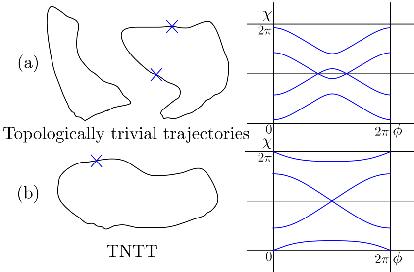
Figure 2.3. Topological classes of trajectories in the space of TTM. A trajectory is topologically non-trivial (TNTT) provided it passes the matrix with two degenerate real eigenvalues odd number of times. Illustration: the dependencies of eigenvalues of the scattering matrix characterizing the SS junction on superconducting phase difference \phi for (a) non-“topological” and (b) “topological” parameter ranges.
