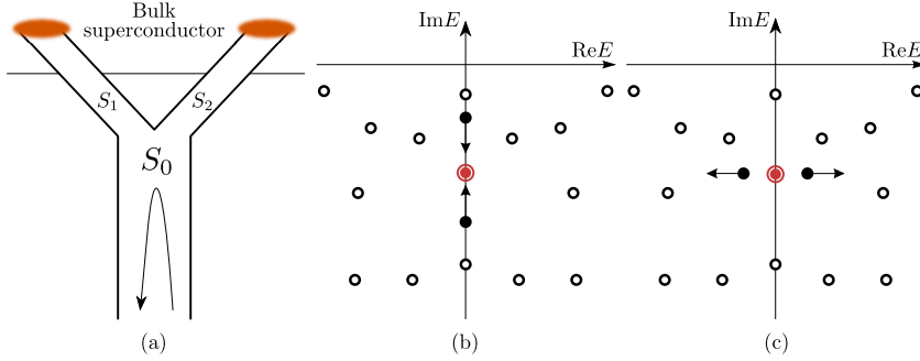
Figure 2.5. (a): Fork SN junction to illustrate topological transitions concerning the resonant poles. (b,c): Configurations of the resonant poles in the complex energy plane (b) before and (c) after a transition. At the transition point, the poles are degenerate (double red circle)
