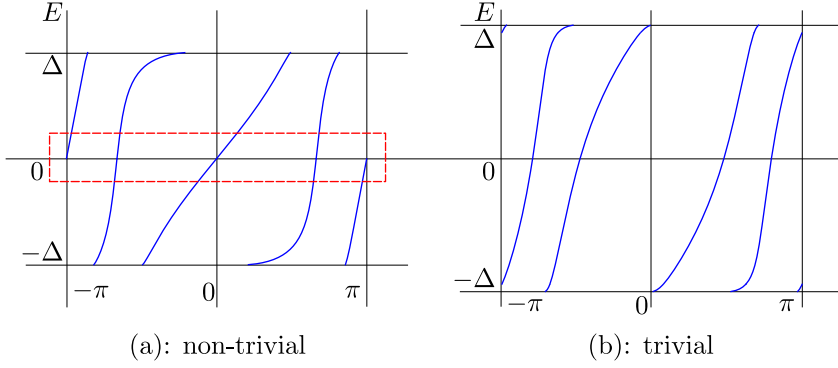
Figure 2.2. Energy dependence of s-matrix eigenvalues. (a) Topologically non-trivial (TNTM) case, corresponding to the “topological” parameter range in [8]. (b) Generic topologically trivial (TTM) case. (Numerical results for the setup in Fig. 1a in the limit L \rightarrow \infty .)
