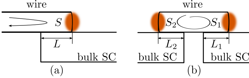
Figure 2.1. Setups to illustrate general topological properties of BdG s-matrices. a. Finite-length wire with strong spin-orbit coupling on the top of superconducting lead forming a SN junction. b. Finite-length wire between two superconductors forming SS junction. Orange ellipses indicate “buried” zero-energy states.
