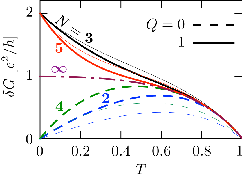
Figure 4.2. Amplitude \delta G of the average zero-voltage conductance peak as a function of (mode-independent) transmission probability T , in symmetry class D (thick curves) and BDI (thin curves) for different number of modes N . The superconductor is topologically trivial when N is even ( Q = 0 , dashed curves) and nontrivial when N is odd ( Q = 1 , solid curves). The dash-dotted curve is the Q -independent large- N limit (4.14).
