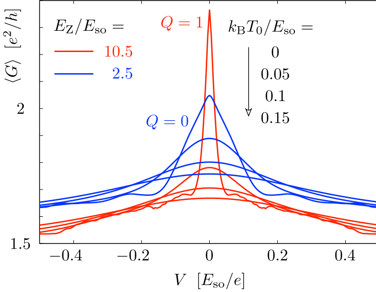
Figure 4.6. Temperature dependence of the conductance peaks from Fig. 4.3b. The four blue curves ( Q = 0 , topologically trivial) correspond from top to bottom to four increasing temperatures, and likewise the four red curves ( Q = 1 , topologically nontrivial).
