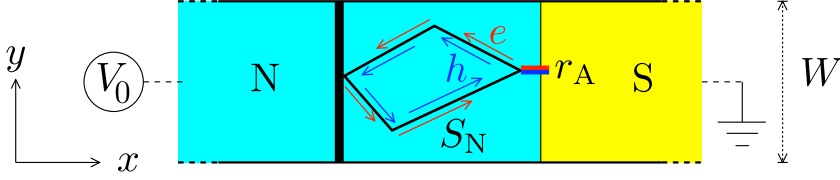
Figure 4.1. A bias voltage V_0 applied to the normal metal (N) drives a current I into the grounded superconductor (S). Electrons and holes ( e, h ) are scattered by disorder or a tunnel barrier in N and converted into each other by Andreev reflection at the NS interface, as described by the scattering matrices S_N and r_A . Particle-hole symmetry ensures that the phase shifts accumulated by e and h along a closed trajectory cancel, irrespective of whether time-reversal symmetry is broken or not. Such phase conjugate series of scattering events permit weak (anti)localization to persist in a magnetic field.
