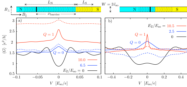
Figure 4.3. Disorder-averaged differential conductance as a function of bias voltage, for a nanowire modeled by the Hamiltonian (4.15). The two panels a) and b) correspond to the two geometries shown to scale above each plot. (The solid vertical line indicates the position of the tunnel barrier, relative to the NS interface; disordered regions are dotted.) Each panel shows data for zero magnetic field (black), and for two nonzero magnetic field values (blue and red). The solid curves are for parallel field B_{\parallel} and the dashed curves for perpendicular field B_{\perp} . The system is topologically trivial ( Q = 0 ) in all cases except for the red solid curves ( Q = 1 ). (The parameter values are listed in Ref. 35.)
