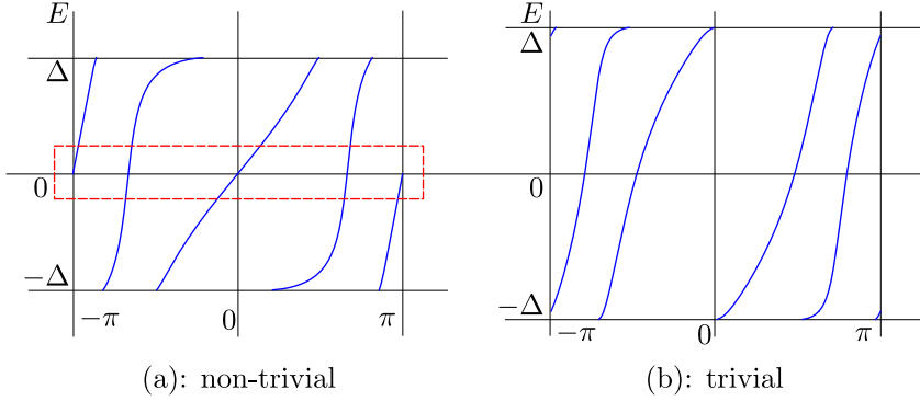
Figure 2.2. Energy dependence of s-matrix eigenvalues. (a) Topologically non-trivial (TNTM) case, corresponding to the “topological” parameter range in [8]. (b) Generic topologically trivial (TTM) case. (Numerical results for the setup in Fig. 1a in the limit L \rightarrow \infty .)
