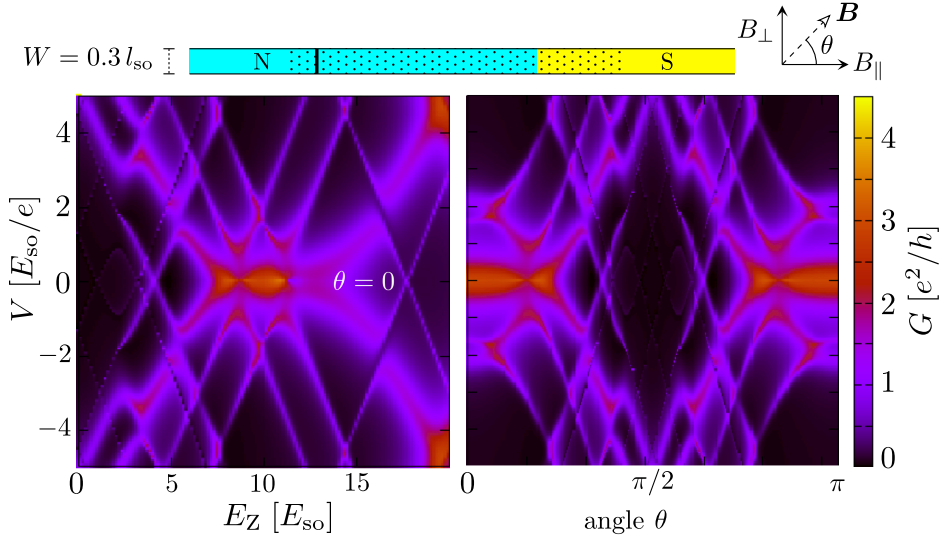
Figure 4.7. Differential conductance for a single disorder realization of a nanowire ( N = 2 spin-resolved modes, parameter values are listed in Ref. 40). The left panel shows the appearance of a zero-voltage peak in a range of magnetic field values, for \mathbf{B} parallel to the wire. The right panel shows the dependence on the orientation of the magnetic field, for a fixed field strength ( E_Z = 10 E_{so} ). The zero-voltage peak vanishes if \mathbf{B} is perpendicular to the wire. This is the same phenomenology as for a Majorana resonance, but here it happens in the topologically trivial phase.
