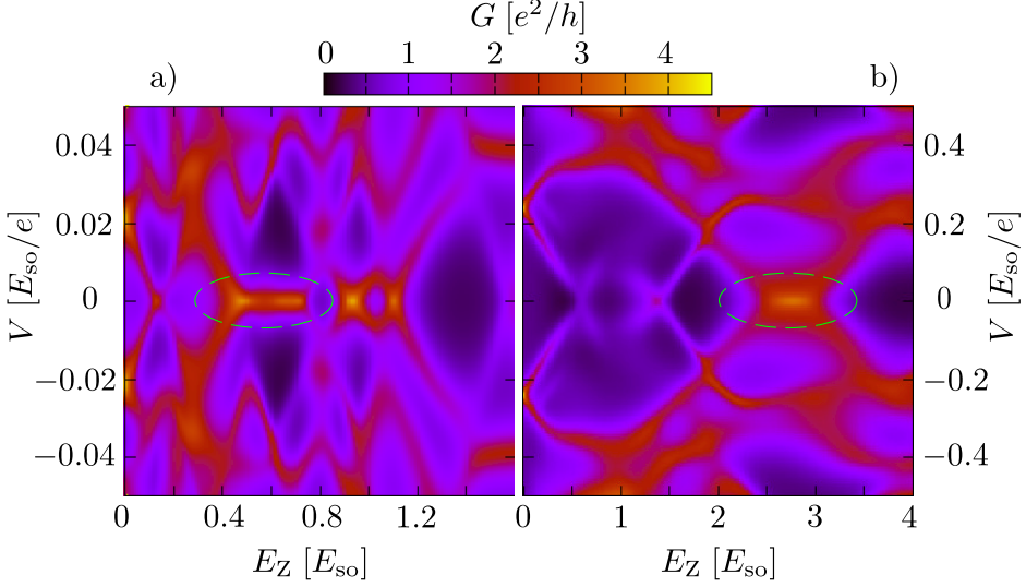
Figure 4.4. Numerical simulation of a nanowire for a single disorder realization (no averaging). The color scale gives the differential conductance as a function of bias voltage (vertical axis) and parallel magnetic field (horizontal axis). The parameters in panels a,b correspond to those in Fig. 4.3a,b, as listed in Ref. 35. The magnetic field range in both panels is in the topologically trivial phase ( Q = 0 ), but still exhibits a conductance peak pinned to zero voltage (green circle).
