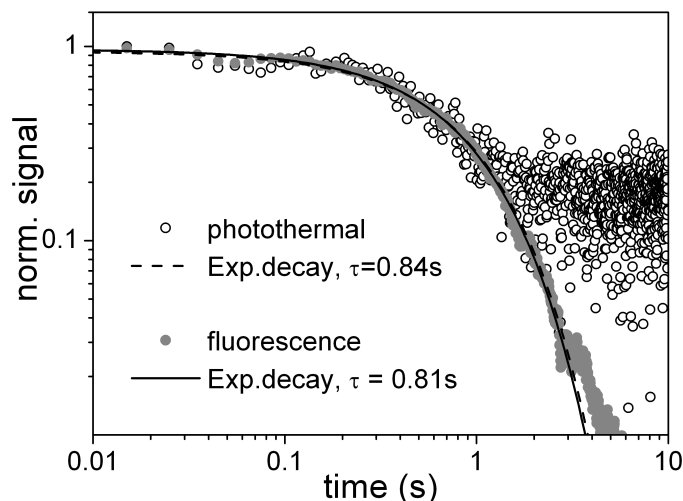
Figure 3.3: Photothermal ( \circ ) and fluorescence ( \bullet ) signal bleaching traces measured on 0.1 wt% fvin NPs on APTES-modified glass in glycerol, shown on a log-log scale. Heating and probe powers were 8.5 \mu\text{W} and 23 \text{ mW} , correspondingly. Characteristic bleaching times estimated from single exponential decay fits are 0.81 \text{ s} , and 0.84 \text{ s} for fluorescence (—) and photothermal (- - -) signals, correspondingly. The normalized signal of about 0.2 is the background level of the photothermal signal.
