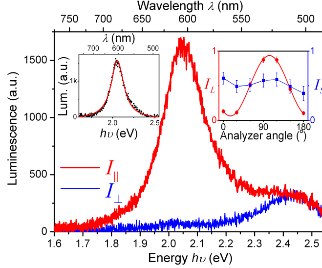
Figure 5.6: Luminescence spectra of a gold nanorod excited by a circular polarized 476 nm laser beam and recorded with a detection polarizer parallel ( I_{||} , red) and perpendicular ( I_{\perp} , blue) to the long axis of the nanorod. Left inset shows the longitudinal component of the luminescence spectrum (black dots) that is obtained after subtracting the luminescence spectrum perpendicular to the long-axis of the nanorod and the Lorentzian-line fit (red). Right inset shows the detection polarization dependence of the long wavelength peak ( I_L , red dots) and the short wavelength peak ( I_S , blue dots).
