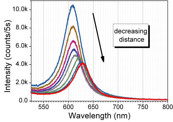
Figure 6.8: The change in the luminescence spectrum of the nanorod when the nanorod is approached with a second glass substrate from the top.
