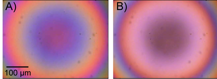
Figure 6.4: Newton's rings formed when the two substrates are in A) optical contact; B) mechanical contact. The contact area should be completely black, but a background from out-of-focus reflections remains.
