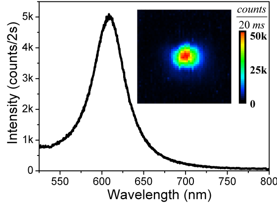
Figure 6.7: Luminescence spectrum of a single gold nanorod. The spectrum was recorded in air on glass substrate with 476\ \text{nm} excitation at 360\ \text{kW}/\text{cm}^2 in 2 s. The plasmon resonance of the nanorod is 608.8\ \text{nm} . The inset shows the luminescence image of the nanorod, which was excited under the same conditions as of the spectrum. The size of the image is 2\ \mu\text{m}^2 \times 2\ \mu\text{m}^2 (20ms/pixel, 40 nm pixel size).
