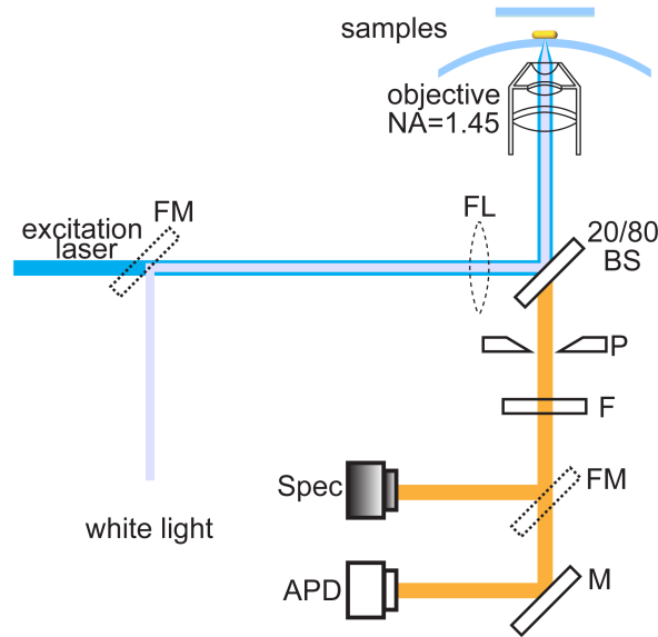
Figure 6.1: Schematic of the experimental setup. FM-flip-mirror; FL-flip-lens; NA-numerical aperture; BS-beam-splitter; P-pinhole; F-filter; M-mirror; APD-Avalanche photodetector; Spec-Spectrometer.
