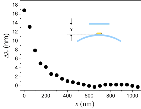
Figure 6.10: The change in the plasmon resonance wavelength ( \Delta\lambda ) as a function of the distance ( s ) between the two substrates.
