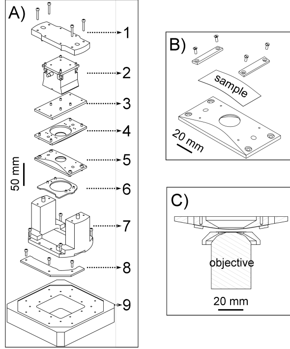
Figure 6.2: A) Components of the variable-distance-cell 1) Aluminum adapter plate to which PI-NanoCube is mounted. 2) PI-NanoCube piezo-stage. 3) Adapter plate for sample mount. 4)Top sample holder. 5)Bottom sample holder. 6)Kinematic platform for bottom sample holder. 7) (Attached) aluminum blocks. 8)Kinematic platform for bridge configuration (1-4,7). 9) PI-MARS piezo-stage. B) Sample holder and cover glass with mounting adapters C) Side view of two sample holders with microscope objective.
