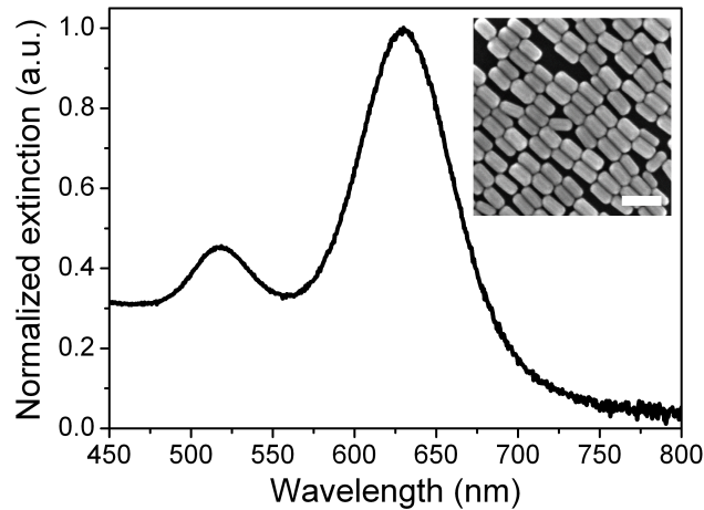
Figure 6.3: Extinction spectrum of gold nanorod suspension in water. There are two peaks. The red-most plasmon resonance corresponds to the longitudinal plasmon resonance of gold nanorods. The blue-most peak is formed by contributions from both transverse plasmon resonance of gold nanorods and residual gold nanospheres in the suspension. The inset shows an SEM image of the sample used in this study. The ensemble average width and length of the nanorods are 30 nm and 65 nm. The scale bar in the inset SEM image is 100 nm.
