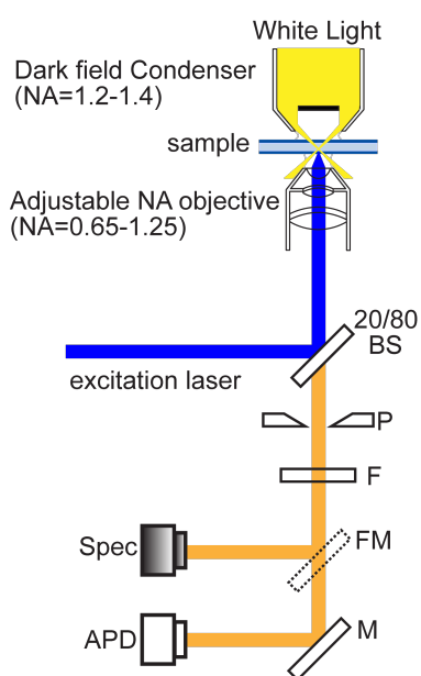
Figure D.2: Schematic of the experimental setup for correlation of scattering and luminescence signals of nanorods. M - mirror, FM - flip mirror, F - filter, P - pinhole, BS - beam splitter, Spec - spectrometer, APD - avalanche photodetector.
