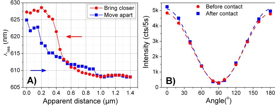
Figure 6.9: (A) The plasmon resonance wavelength \lambda_{res} as a function of the apparent distance between the two substrates. (B) Longitudinal plasmon resonance intensity as a function of the analyzer angle. For both images red-circles represent data which are obtained while decreasing the distance between the two substrates. The blue-square data is of experiment when the top substrate was retracted.
