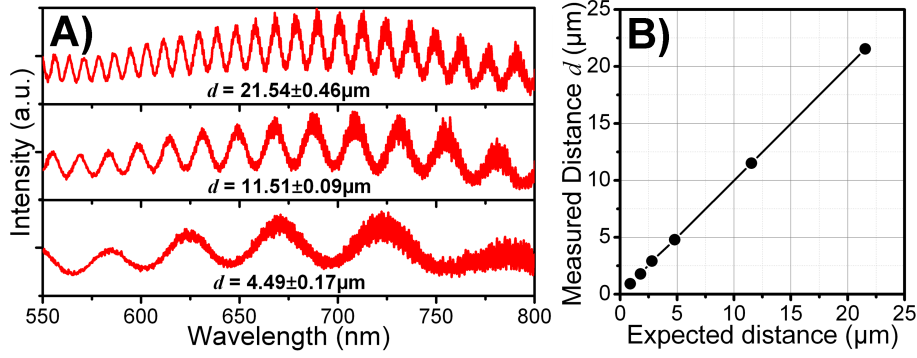
Figure 6.5: (A) Fringes of the reflected white light from the friction cell at different air-gap thickness. Distances (B) Characterization of the piezo stage movement and the distance measurement.
