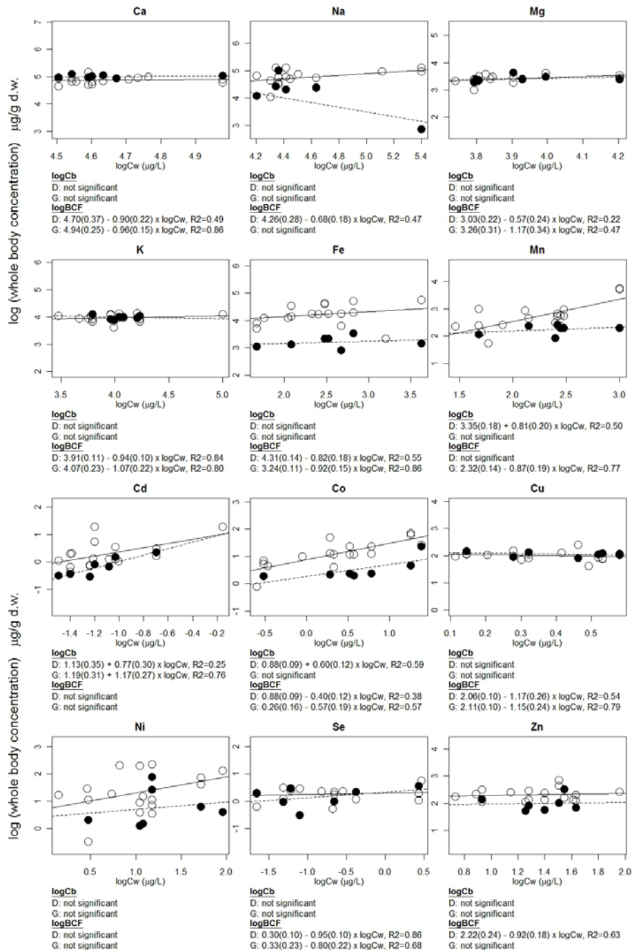
Figure 2.2 Whole-body concentrations of metals in D. magna ( \circ ) and G. roeseli ( \bullet ) related to dissolved metal concentrations (Cw) in twelve natural surface waters. Regression functions of logCb-logCw and logBCF-logCw are printed below the figures, with standard error of the estimated coefficients between brackets.
