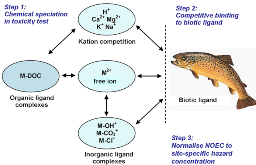
Figure 1.1 Schematic of biotic ligand binding
